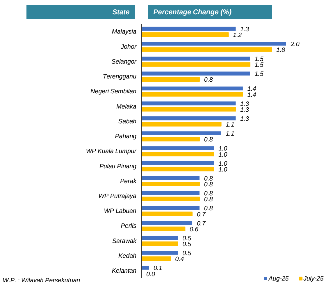
Chart 7 Inflation by State, July 2025 & Aug 2025
