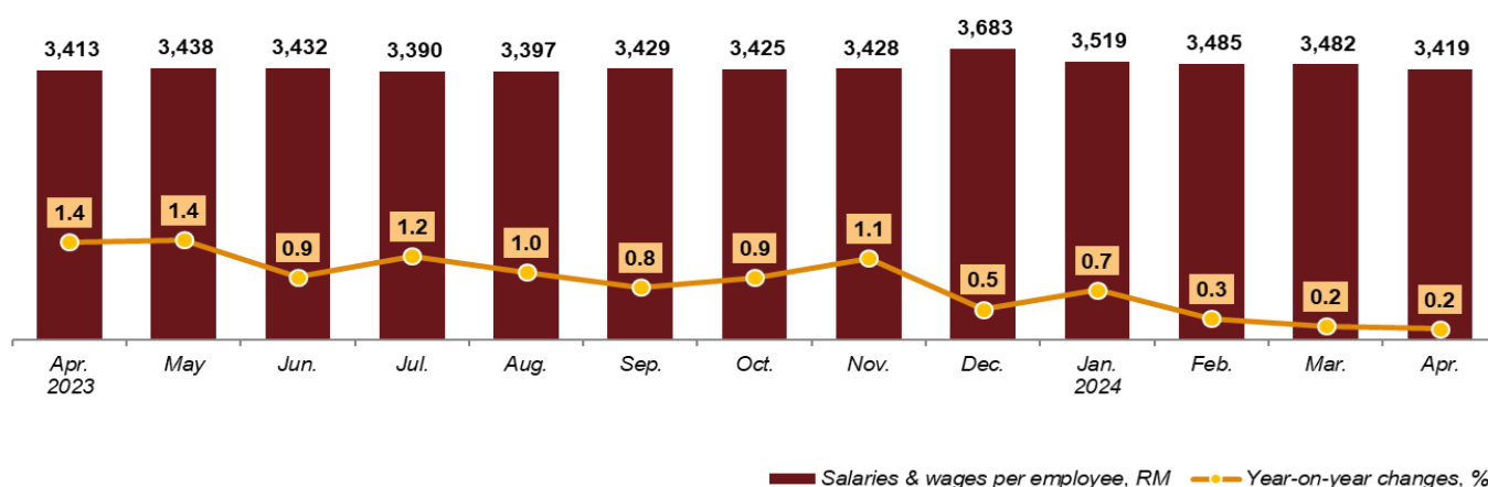
Chart 3: Salaries & Wages per Employee in Manufacturing Sector, April 2023 – April 2024
