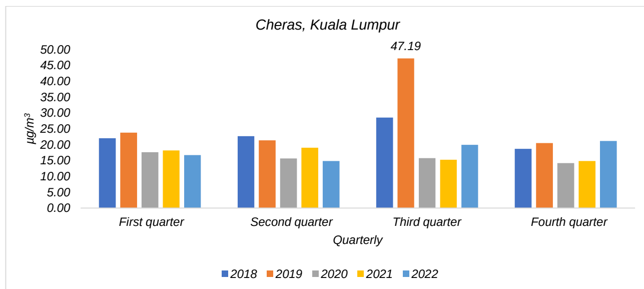
Carta 1.2: Quarterly average concentration of Particulate Matter ( PM_{2.5} ) in the air, Cheras, Kuala Lumpur station, 2018-2022
