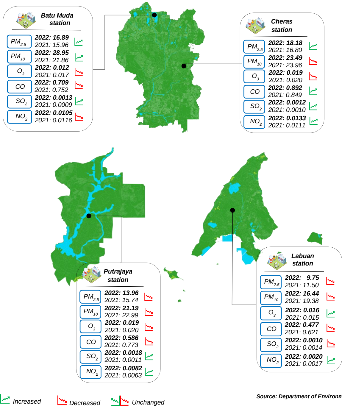
Exhibit 1.3: Summary of air pollutants statistics by station, Wilayah Persekutuan, 2021 and 2022
