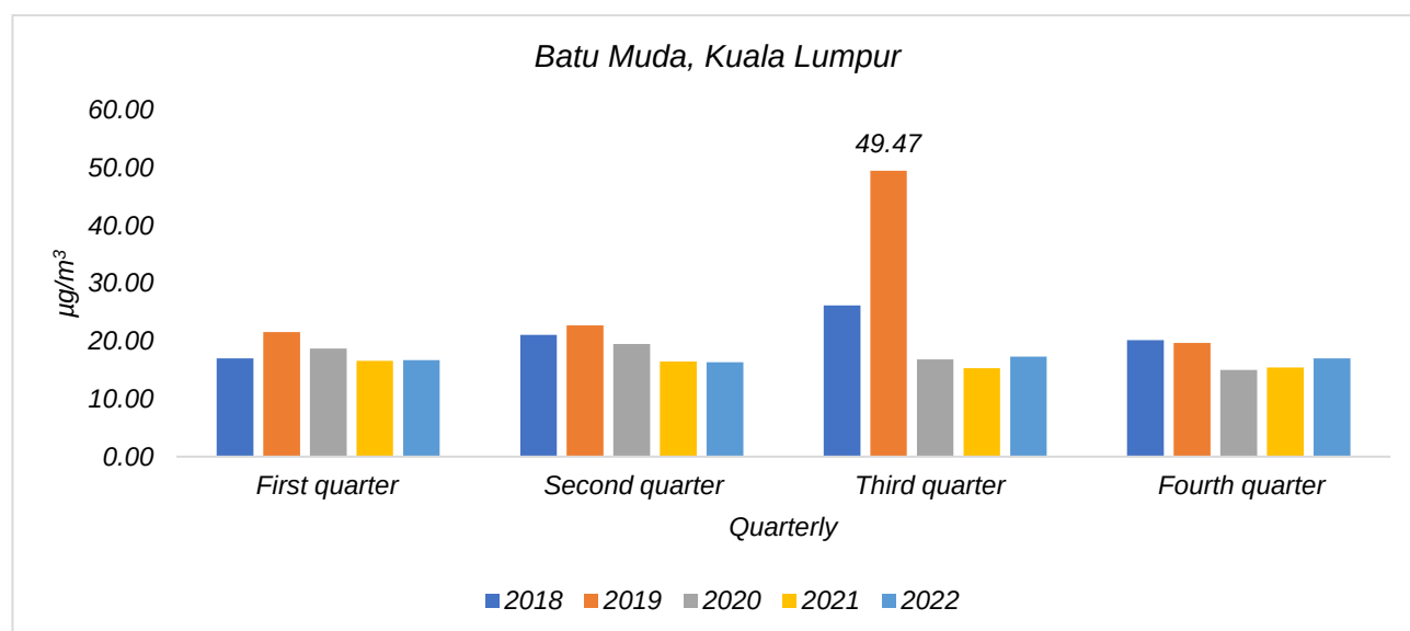
Chart 1.1: Quarterly average concentration of Particulate Matter ( PM_{2.5} ) in the air, Batu Muda, Kuala Lumpur station, 2018-2022
