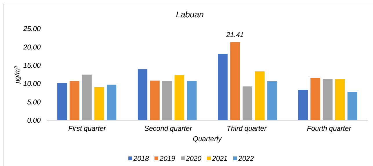
Carta 1.3: Quarterly average concentration of Particulate Matter ( PM_{2.5} ) in the air, Labuan station, 2018-2022
