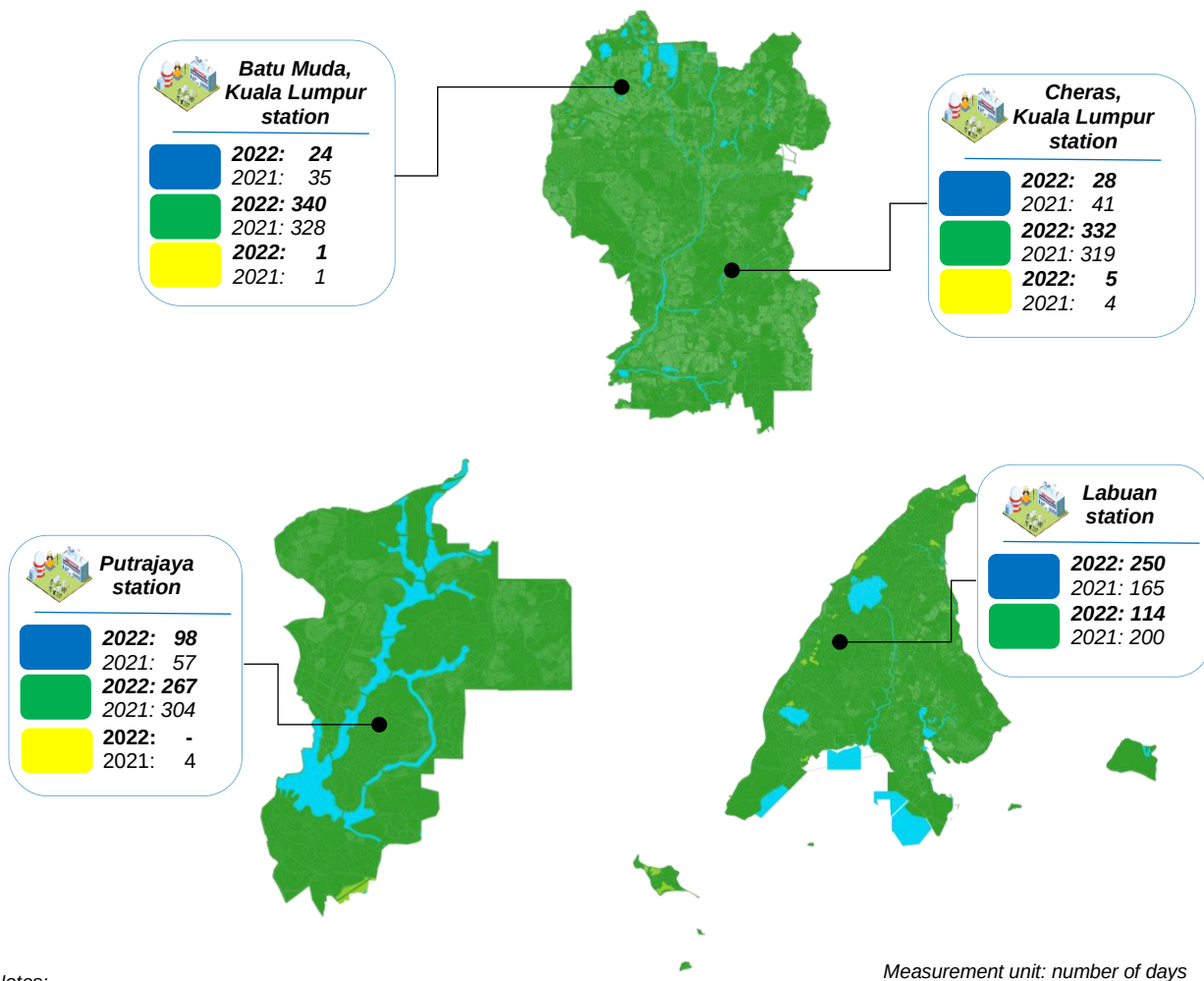
Exhibit 1.5: Status of air quality by station, Wilayah Persekutuan, 2021 and 2022
