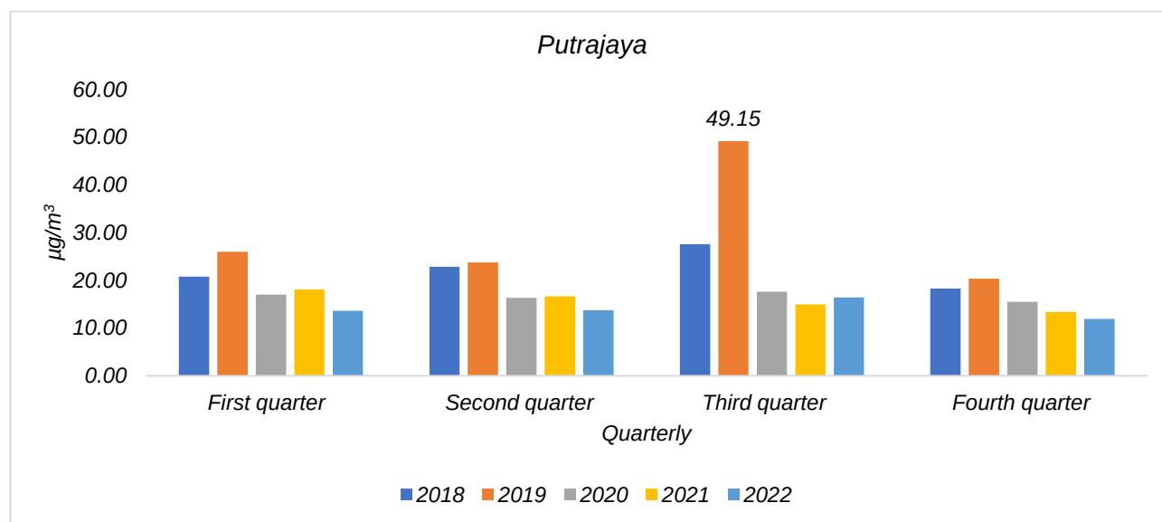
Carta 1.4: Quarterly average concentration of Particulate Matter ( PM_{2.5} ) in the air, Putrajaya station, 2018-2022
