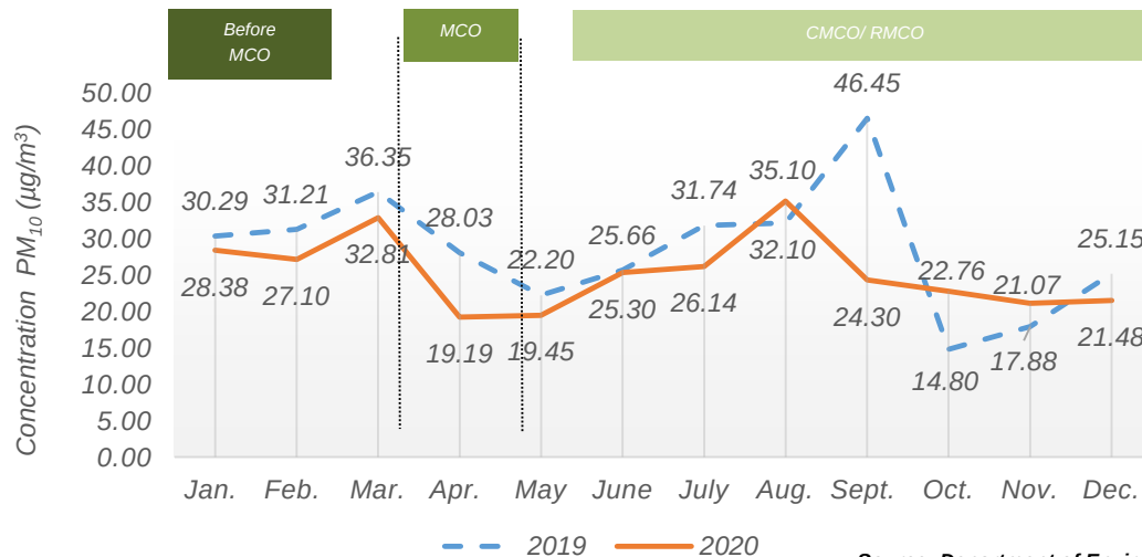
Chart 1.3: Monthly average concentration of PM 10 in the air, Seberang Jaya station, Pulau Pinang, 2019 and 2020
