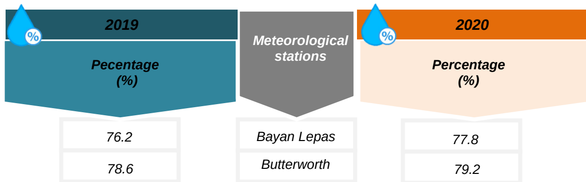
Exhibit 1.3: Mean relative humidity at meteorological stations, Pulau Pinang, 2019 and 2020
