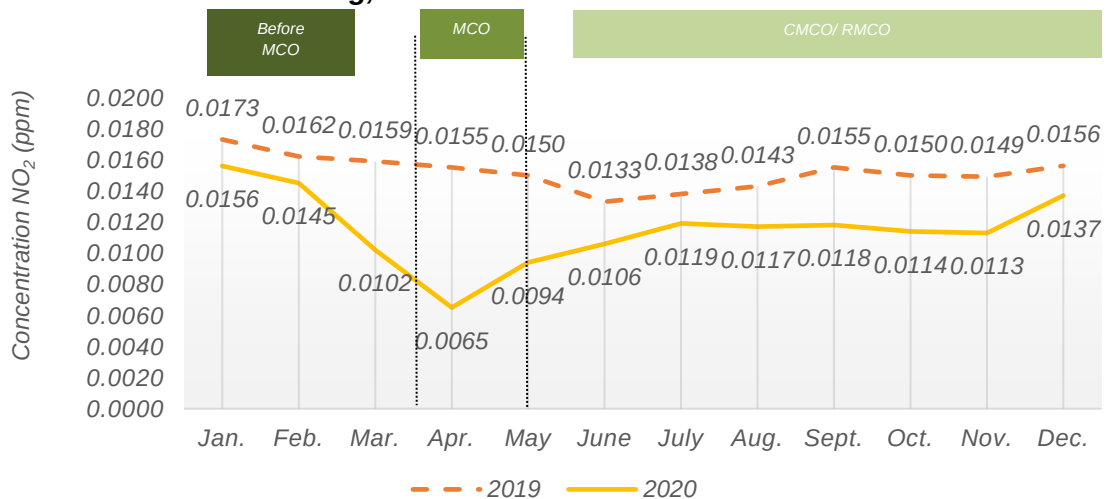
Chart 1.23: Monthly average concentration of NO 2 in the air, Seberang Jaya station, Pulau Pinang, 2019 and 2020
