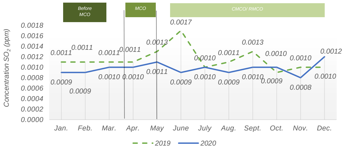
Chart 1.19: Monthly average concentration of SO 2 in the air, Seberang Jaya station, Pulau Pinang, 2019 and 2020
