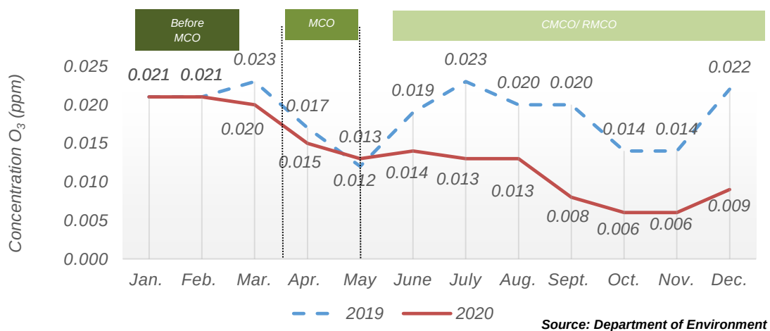
Chart 1.11: Monthly average concentration of O 3 in the air, Seberang Jaya station, Pulau Pinang, 2019 and 2020
