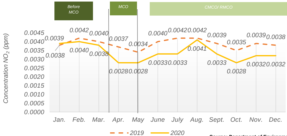
Chart 1.21: Monthly average concentration of NO 2 in the air, Balik Pulau station, Pulau Pinang, 2019 and 2020
