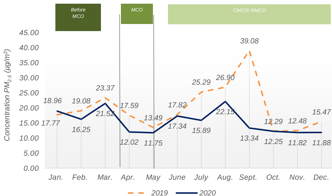
Chart 1.6: Monthly average concentration of PM_{2.5} in the air, Perai station, Pulau Pinang, 2019 and 2020
