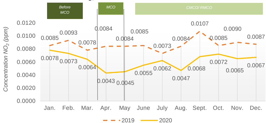
Chart 1.24: Monthly average concentration of NO 2 in the air, USM station, Pulau Pinang, 2019 and 2020
