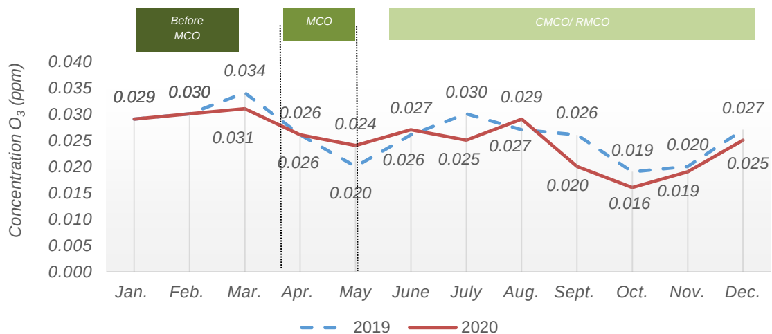
Chart 1.12: Monthly average concentration of O 3 in the air, USM station, Pulau Pinang, 2019 and 2020
