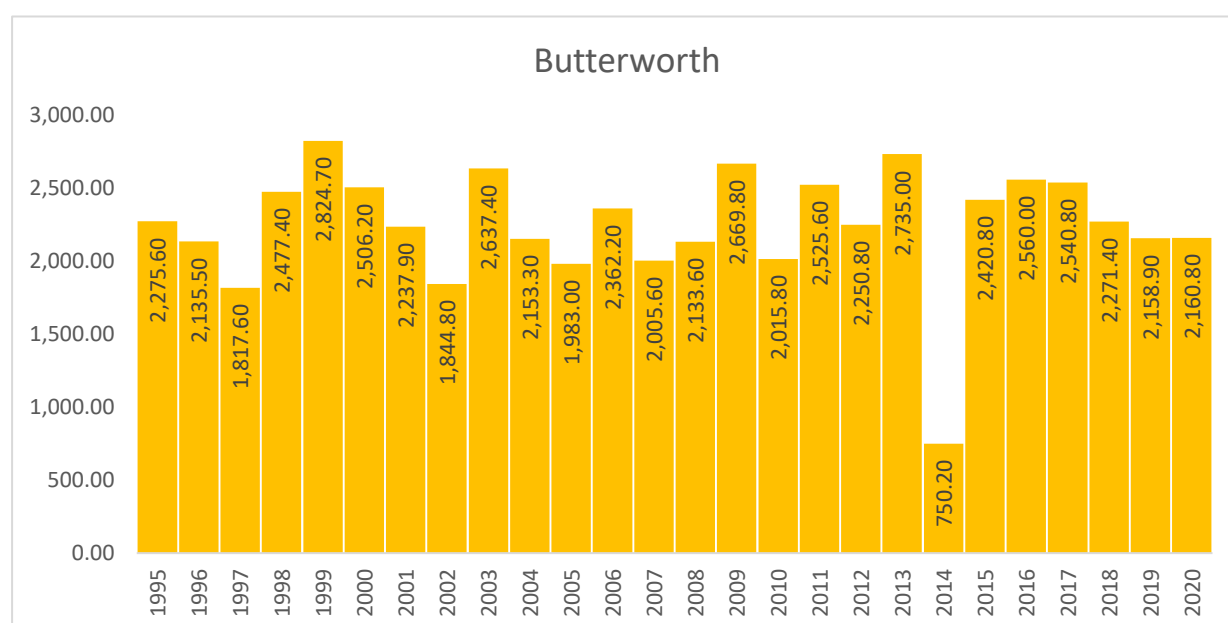
Chart 1.2: Rainfall distribution at Butterworth meteorological station, Pulau Pinang, 1995-2020
