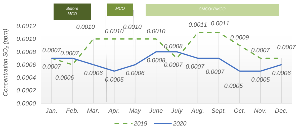
Chart 1.18: Monthly average concentration of SO 2 in the air, Perai station, Pulau Pinang, 2019 and 2020
