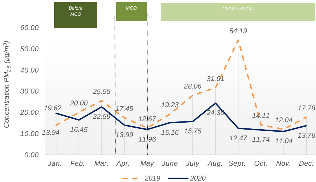
Chart 1.5: Monthly average concentration of PM_{2.5} in the air, Balik Pulau station, Pulau Pinang, 2019 and 2020
