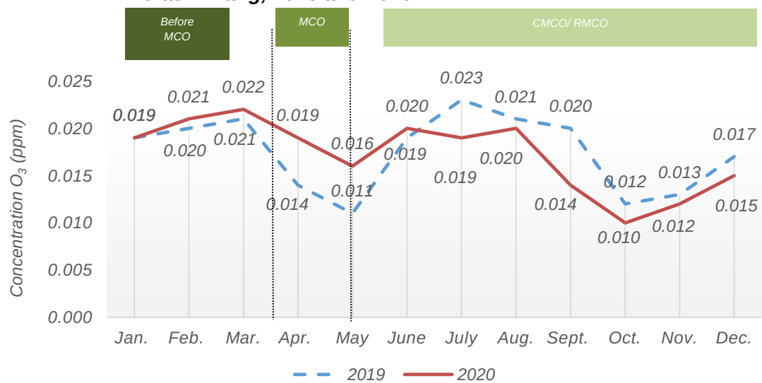
Chart 1.11: Monthly average concentration of O 3 in the air, Seberang Jaya station, Pulau Pinang, 2019 and 2020
