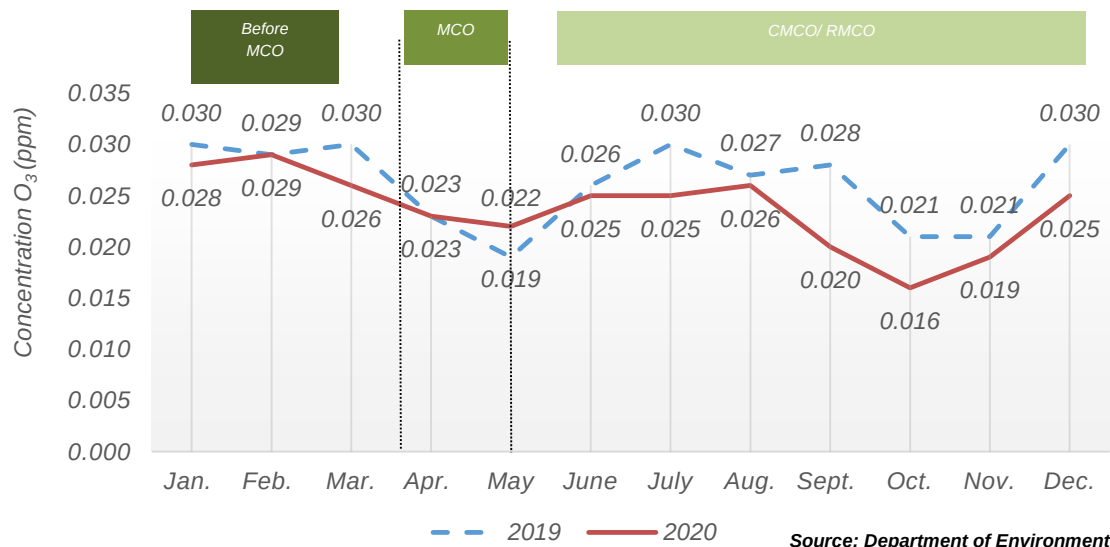
Chart 1.10: Monthly average concentration of O 3 in the air, Perai station, Pulau Pinang, 2019 and 2020
