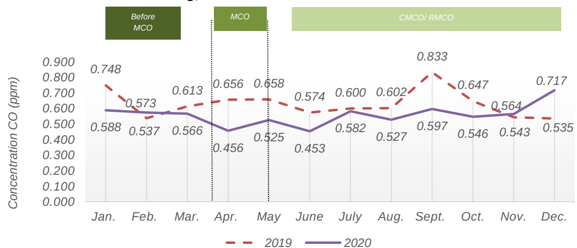
Chart 1.16: Monthly average concentration of CO in the air, USM station, Pulau Pinang, 2019 and 2020
