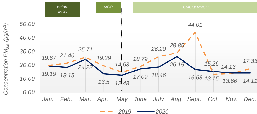
Chart 1.7: Monthly average concentration of PM 2.5 in the air, Seberang Jaya station, Pulau Pinang, 2019 and 2020
