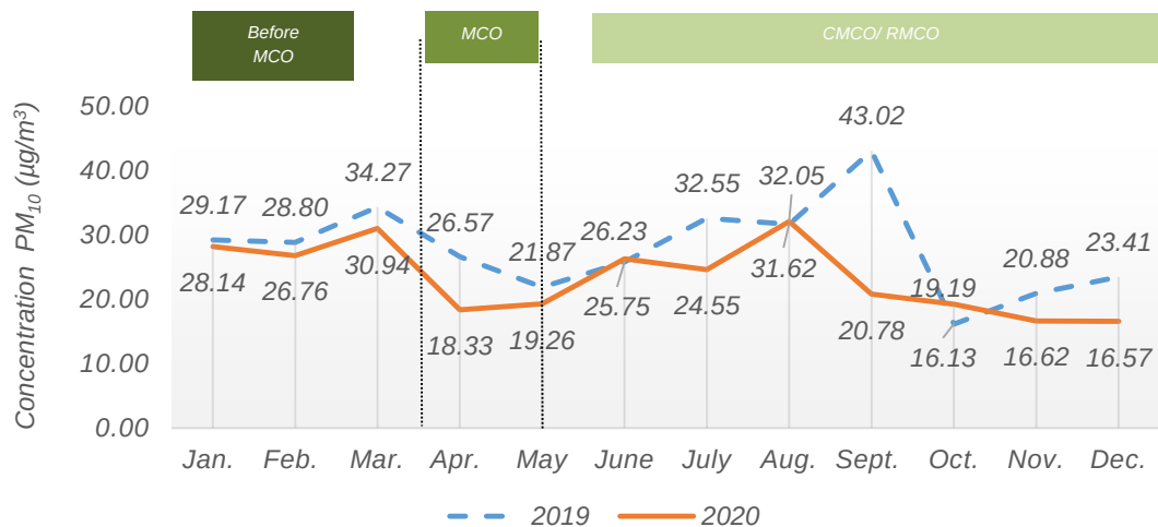
Chart 1.2: Monthly average concentration of PM 10 in the air, Perai station, Pulau Pinang, 2019 and 2020
