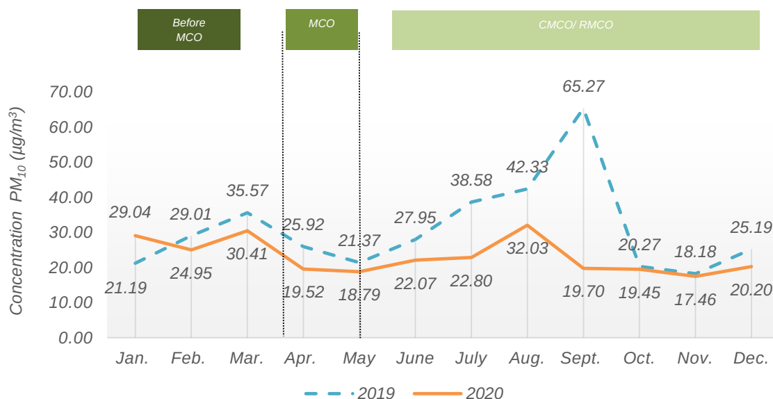
Chart 1.1: Monthly average concentration of PM_{10} in the air, Balik Pulau station, Pulau Pinang, 2019 and 2020
