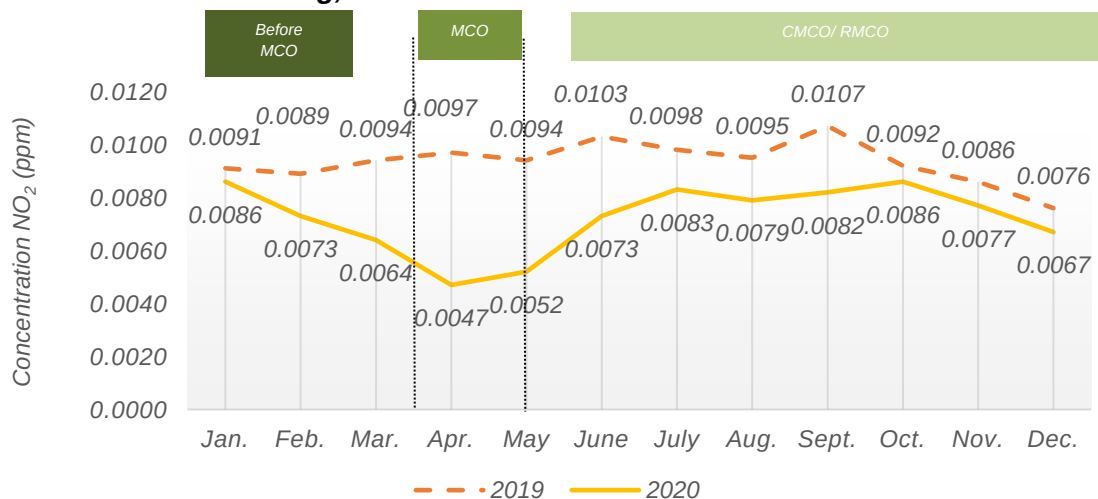
Chart 1.22: Monthly average concentration of NO 2 in the air, Seberang Perai station, Pulau Pinang, 2019 and 2020
