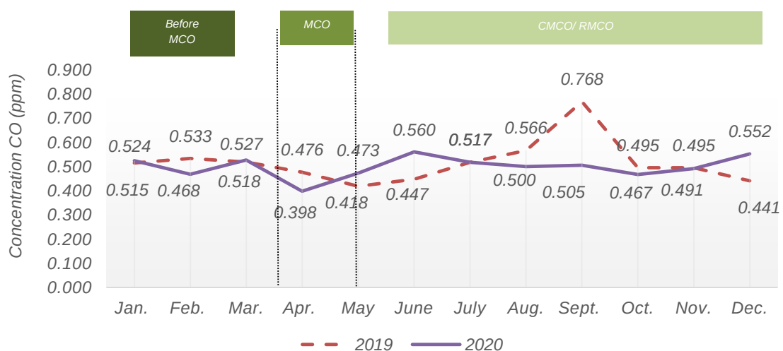
Chart 1.13: Monthly average concentration of CO in the air, Balik Pulau station, Pulau Pinang, 2019 and 2020
