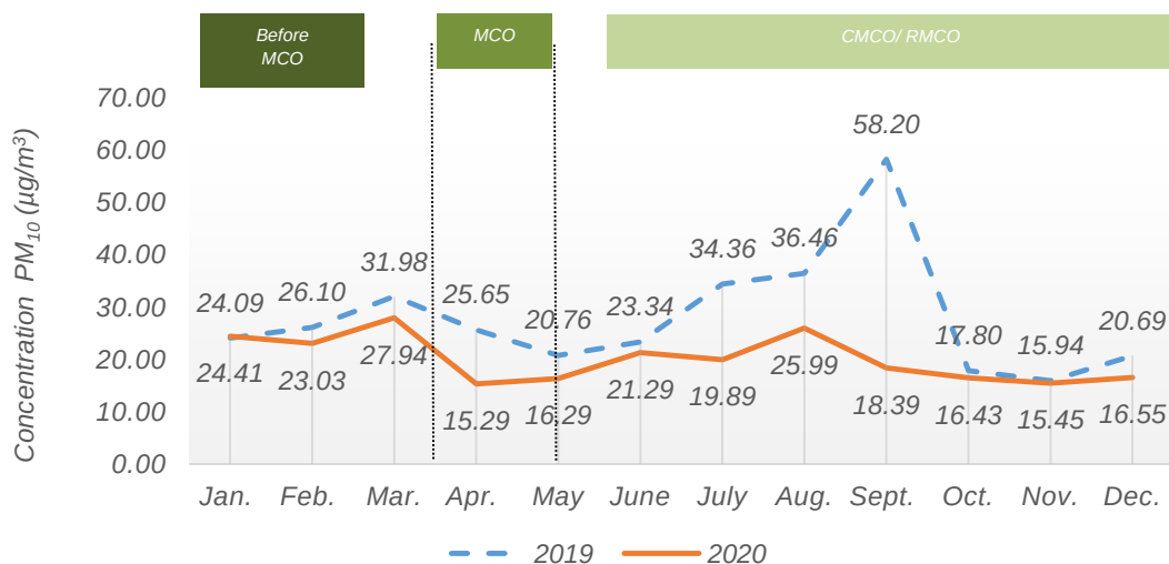
Chart 1.4: Monthly average concentration of PM 10 in the air, USM station, Pulau Pinang, 2019 and 2020
