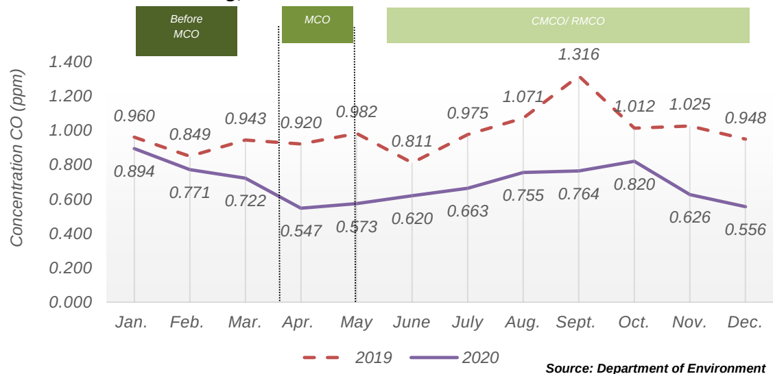
Chart 1.15: Monthly average concentration of CO in the air, Seberang Jaya station, Pulau Pinang, 2019 and 2020
