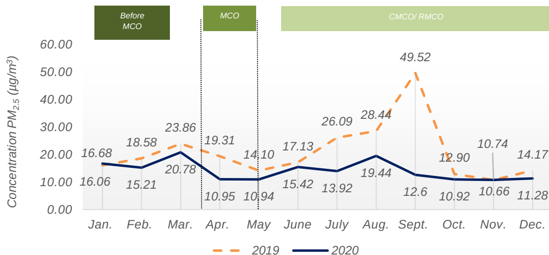
Chart 1.8: Monthly average concentration of PM 2.5 in the air, USM station, Pulau Pinang, 2019 and 2020
