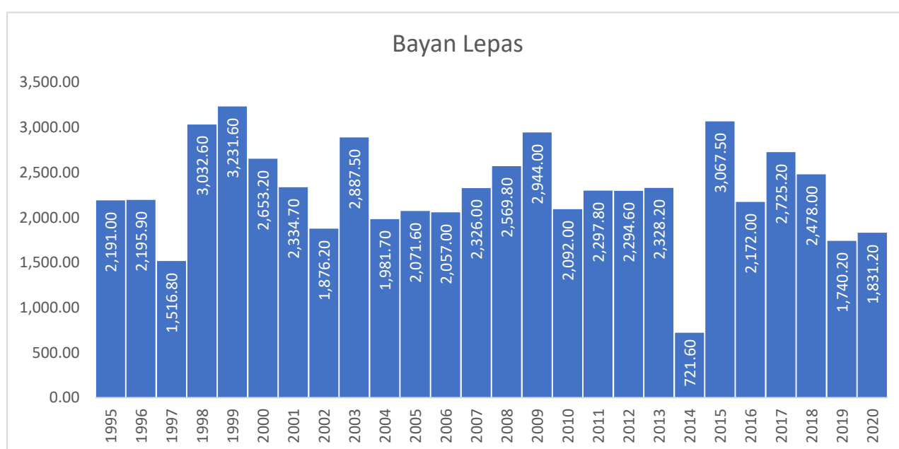
Chart 1.1: Rainfall distribution at Bayan Lepas meteorological station, Pulau Pinang, 1995-2020
