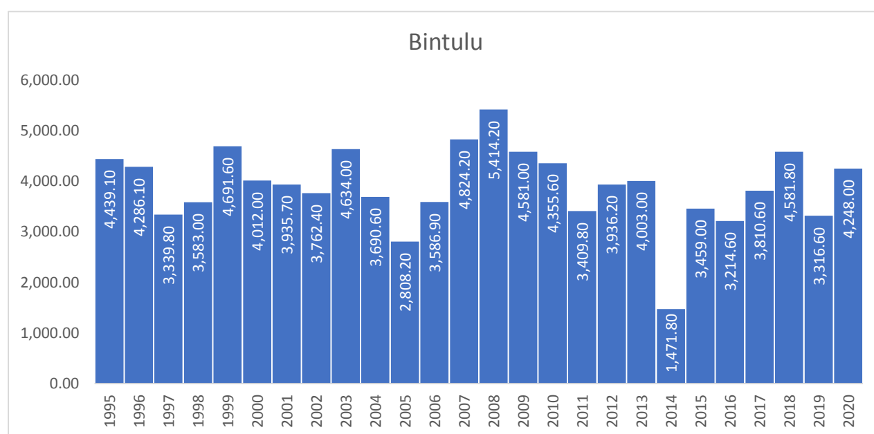
Chart 1.1: Rainfall distribution at Bintulu meteorological station, Sarawak, 1995-2020
