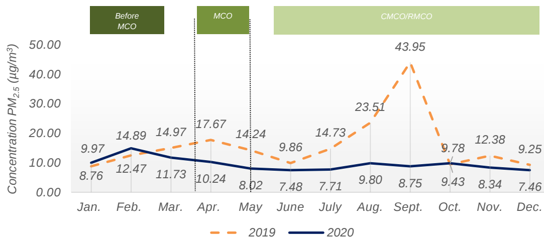
Chart 1.20: Monthly average concentration of PM 2.5 in the air, Samalaju station, Sarawak, 2019 and 2020
