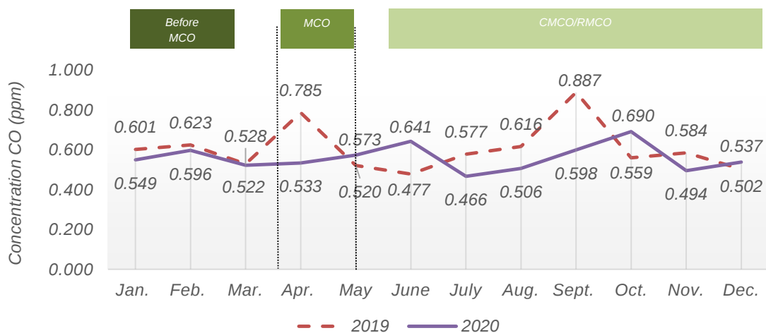
Chart 1.31: Monthly average concentration of CO in the air, Miri station, Sarawak, 2019 and 2020
