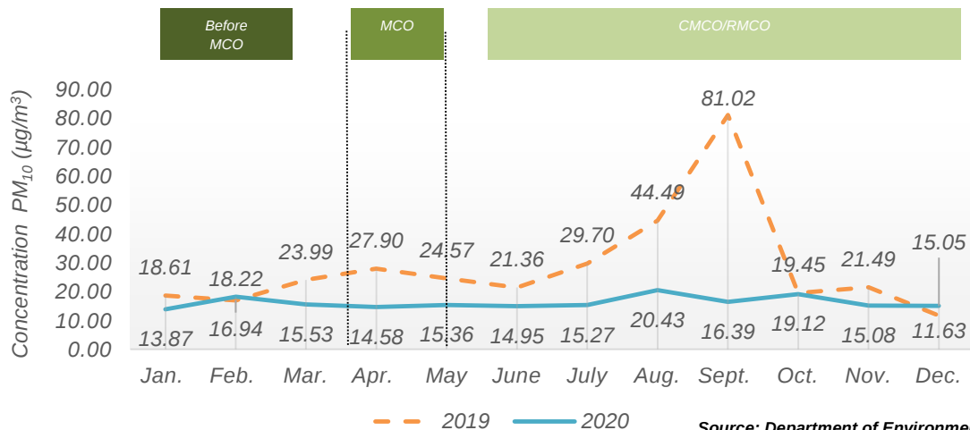
Chart 1.7: Monthly average concentration of PM_{10} in the air, Mukah station, Sarawak, 2019 and 2020
