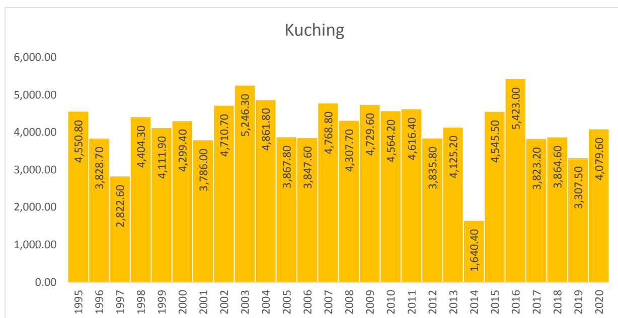
Chart 1.2: Rainfall distribution at Kuching meteorological station, Sarawak, 1995-2020
