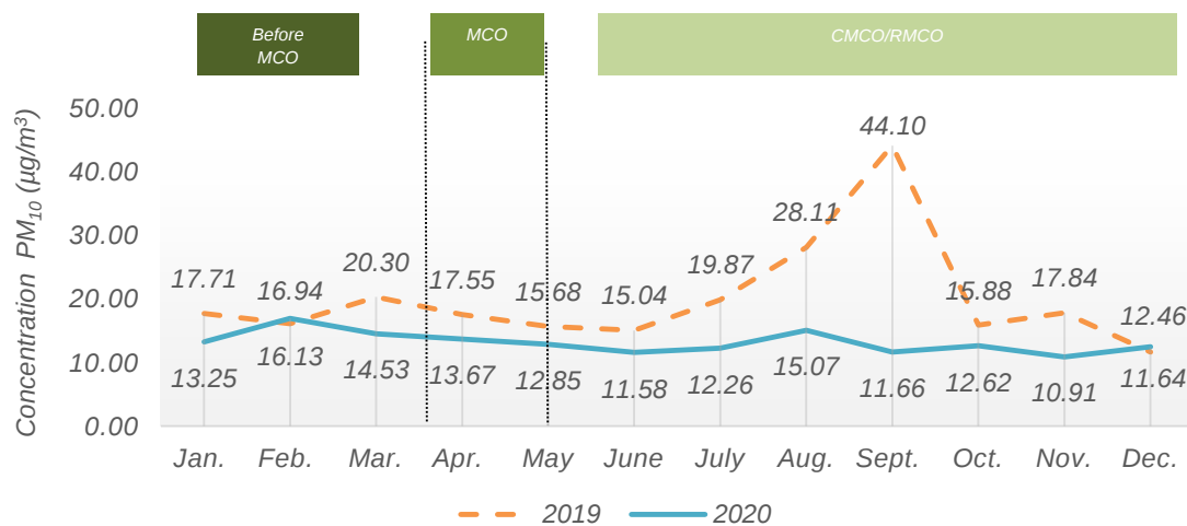
Chart 1.3: Monthly average concentration of PM 10 in the air, Kapit station, Sarawak, 2019 and 2020
