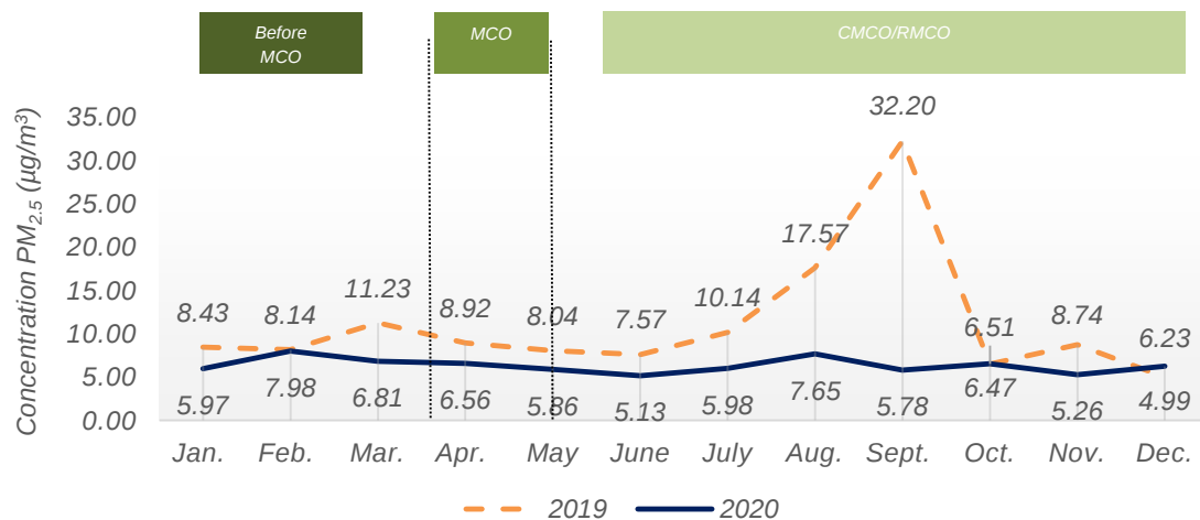
Chart 1.15: Monthly average concentration of PM 2.5 in the air, Kapit station, Sarawak, 2019 and 2020
