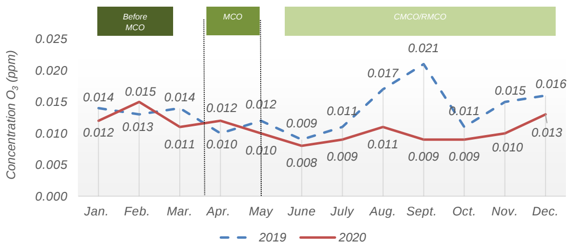
Chart 1.26: Monthly average concentration of O_3 in the air, Kuching station, Sarawak, 2019 and 2020
