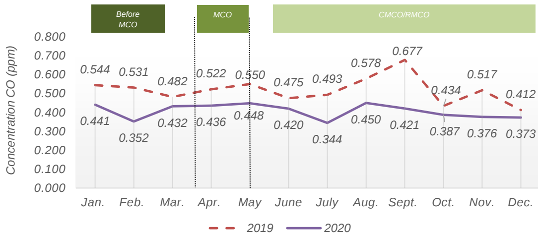
Chart 1.29: Monthly average concentration of CO in the air, Bintulu station, Sarawak, 2019 and 2020
