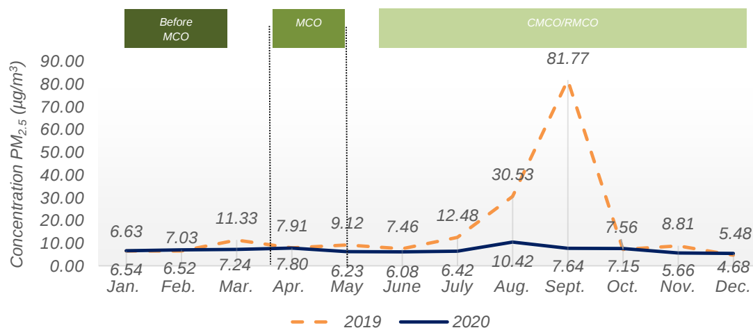
Chart 1.21: Monthly average concentration of PM 2.5 in the air, Samarahan station, Sarawak, 2019 and 2020
