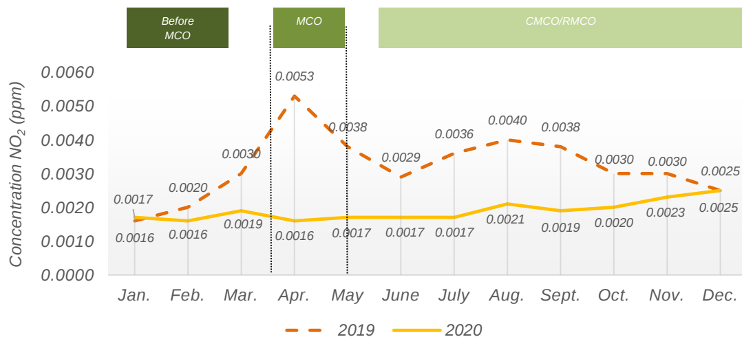
Chart 1.41: Monthly average concentration of NO 2 in the air, Samalaju station, Sarawak, 2019 and 2020
