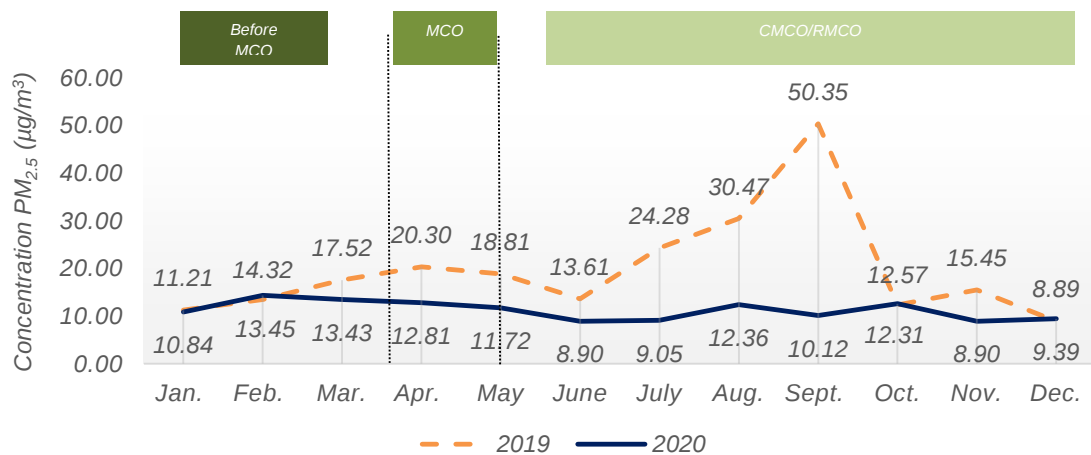
Chart 1.13: Monthly average concentration of PM 2.5 in the air, Bintulu station, Sarawak, 2019 and 2020
