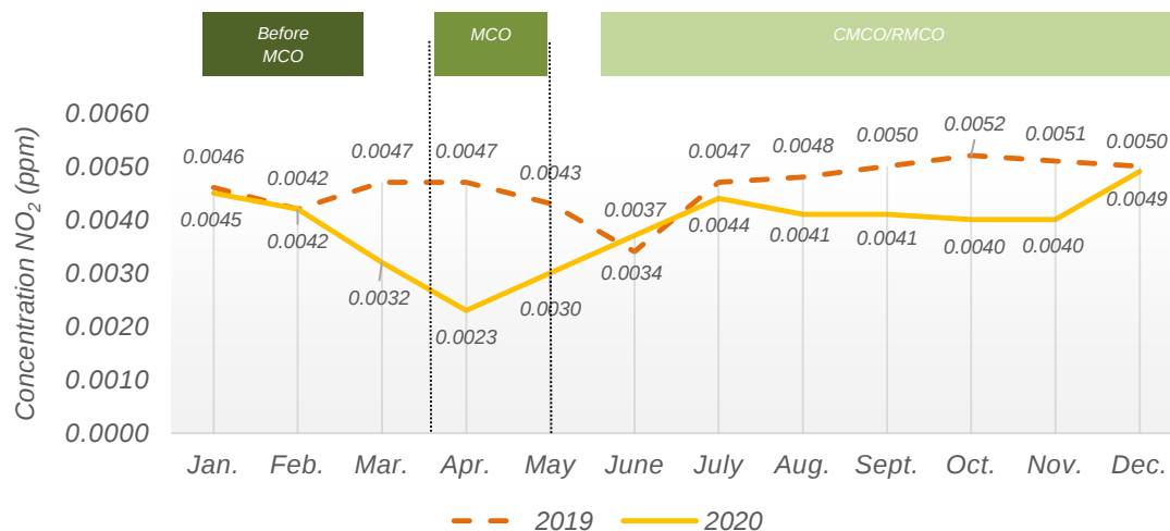
Chart 1.42: Monthly average concentration of NO 2 in the air, Sibu station, Sarawak, 2019 and 2020
