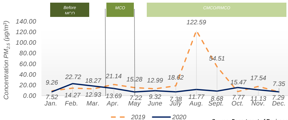
Chart 1.14: Monthly average concentration of PM 2.5 in the air, ILP Miri station, Sarawak, 2019 and 2020
