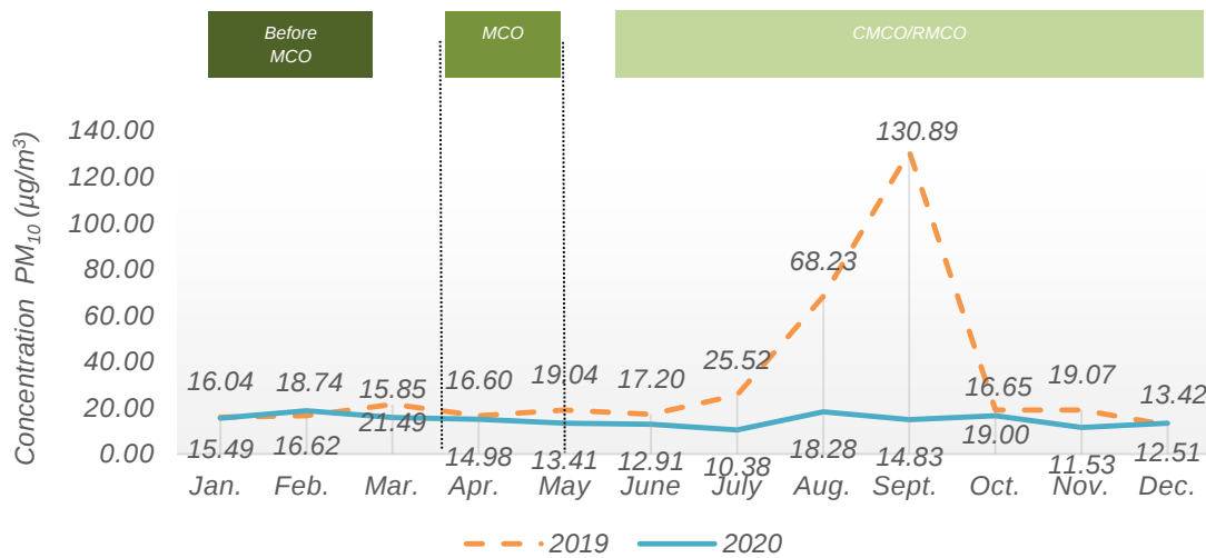
Chart 1.2: Monthly average concentration of PM 10 in the air, ILP Miri station, Sarawak, 2019 and 2020
