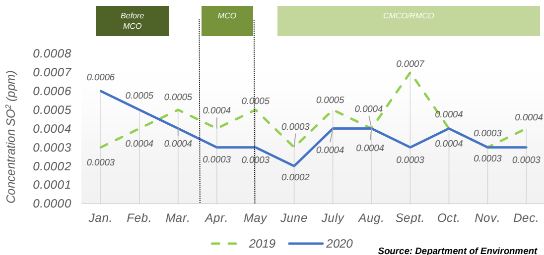
Chart 1.33: Monthly average concentration of SO 2 in the air, Bintulu station, Sarawak, 2019 and 2020
