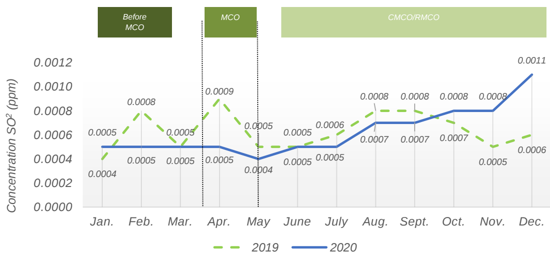
Chart 1.35: Monthly average concentration of SO 2 in the air, Miri station, Sarawak, 2019 and 2020
