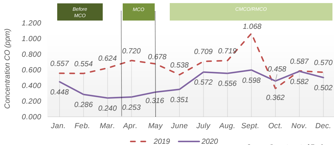
Chart 1.32: Monthly average concentration of CO in the air, Sibul station, Sarawak, 2019 and 2020
