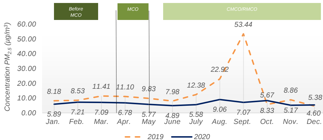
Chart 1.19: Monthly average concentration of PM 2.5 in the air, Mukah station, Sarawak, 2019 and 2020
