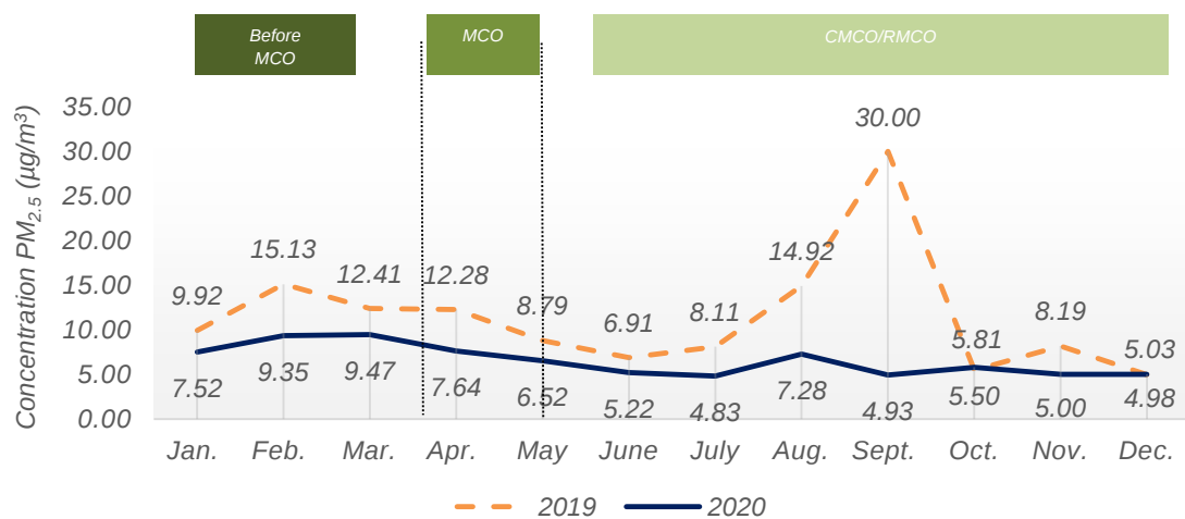
Chart 1.17: Monthly average concentration of PM 2.5 in the air, Limbang station, Sarawak, 2019 and 2020
