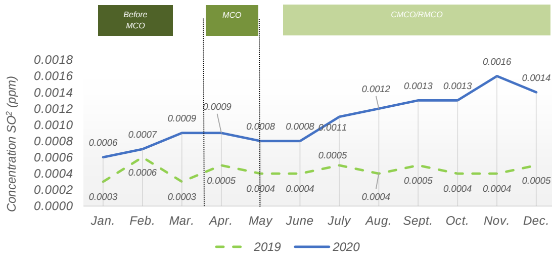
Chart 1.37: Monthly average concentration of SO 2 in the air, Sibu station, Sarawak, 2019 and 2020
