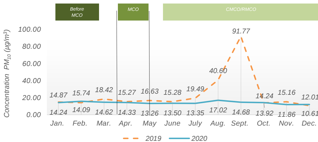
Chart 1.9: Monthly average concentration of PM_{10} in the air, Samarahan station, Sarawak, 2019 and 2020
