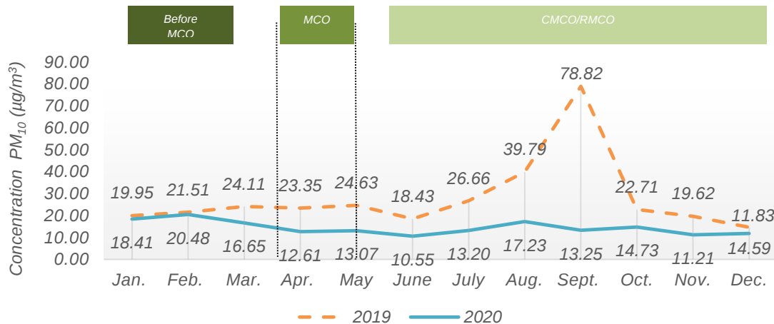
Chart 1.5: Monthly average concentration of PM_{10} in the air, Limbang station, Sarawak, 2019 and 2020
