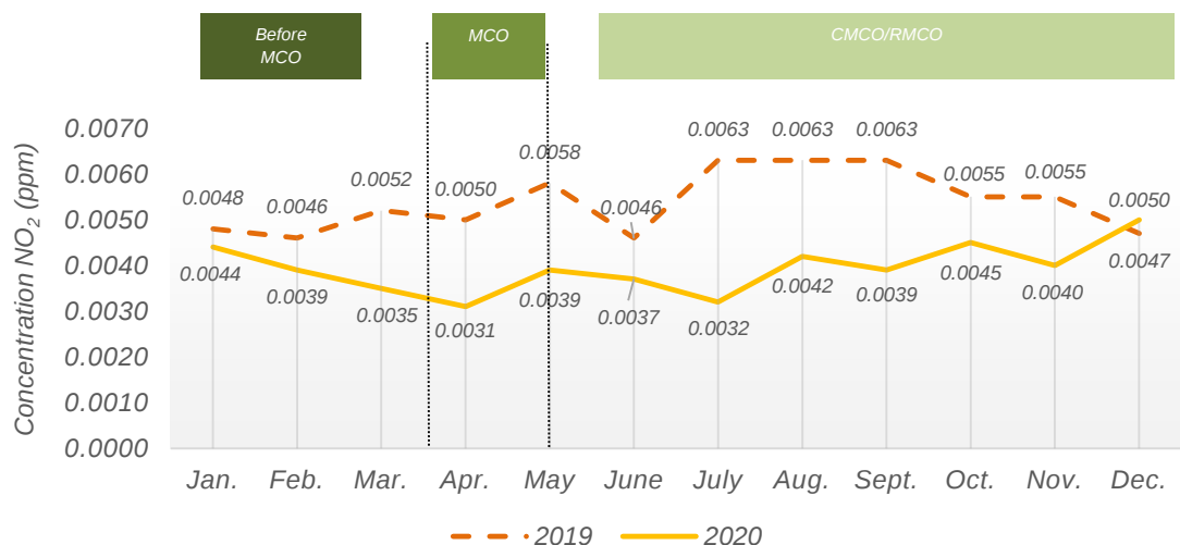
Chart 1.38: Monthly average concentration of NO 2 in the air, Bintulu station, Sarawak, 2019 and 2020
