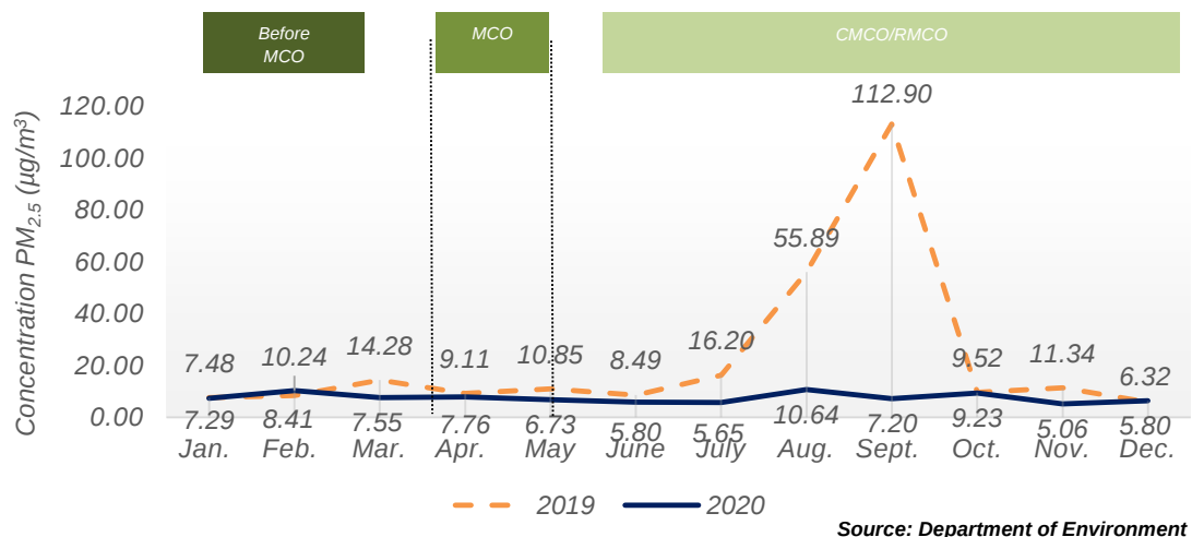
Chart 1.24: Monthly average concentration of PM 2.5 in the air, Sri Aman station, Sarawak, 2019 and 2020
