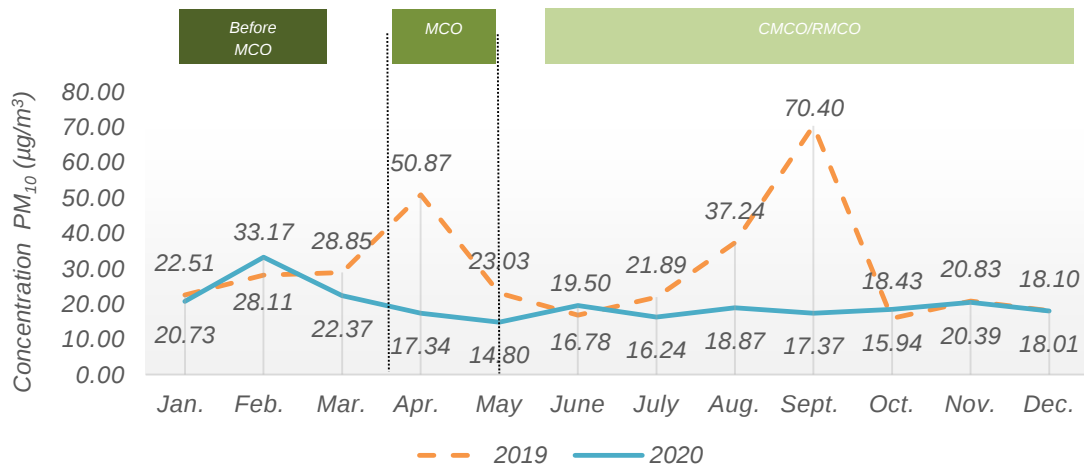
Chart 1.6: Monthly average concentration of PM_{10} in the air, Miri station, Sarawak, 2019 and 2020
