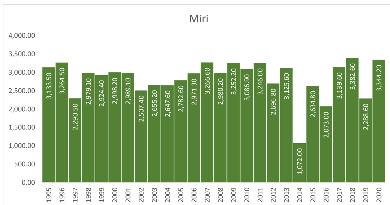
Chart 1.3: Rainfall distribution at Miri meteorological station, Sarawak, 1995-2020
