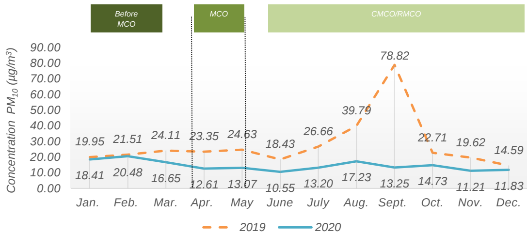
Chart 1.11: Monthly average concentration of PM 10 in the air, Sibu station, Sarawak, 2019 and 2020
