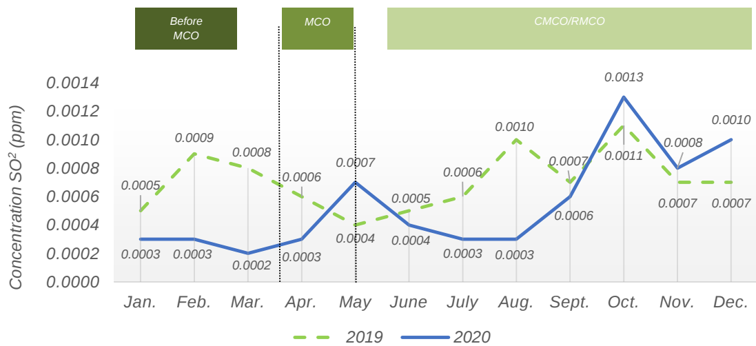
Chart 1.34: Monthly average concentration of SO 2 in the air, Kuching station, Sarawak, 2019 and 2020
