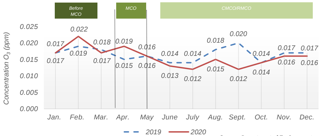
Chart 1.27: Monthly average concentration of O 3 in the air, Miri station, Sarawak, 2019 and 2020
