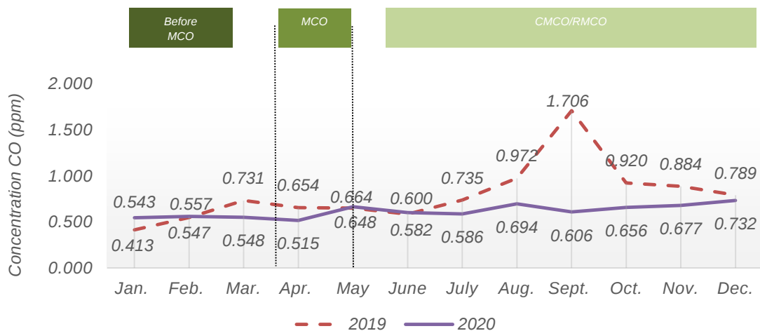
Chart 1.30: Monthly average concentration of CO in the air, Kuching station, Sarawak, 2019 and 2020
