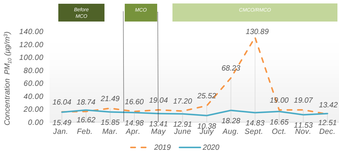
Chart 1.12: Monthly average concentration of PM 10 in the air, Sri Aman station, Sarawak, 2019 and 2020
