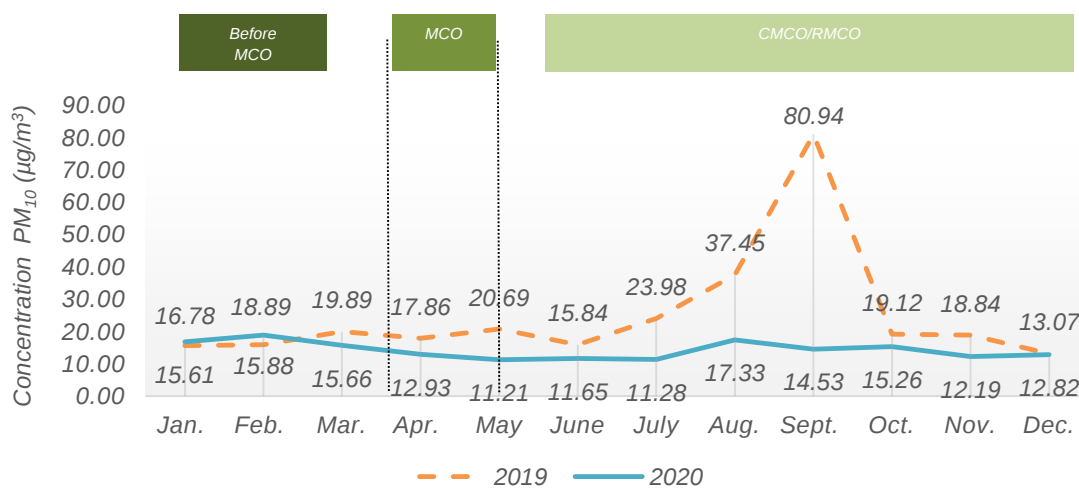
Chart 1.10: Monthly average concentration of PM_{10} in the air, Sarikei station, Sarawak, 2019 and 2020
