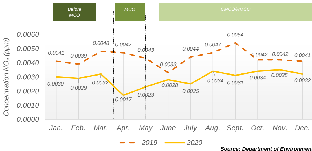
Chart 1.40: Monthly average concentration of NO 2 in the air, Miri station, Sarawak, 2019 and 2020
