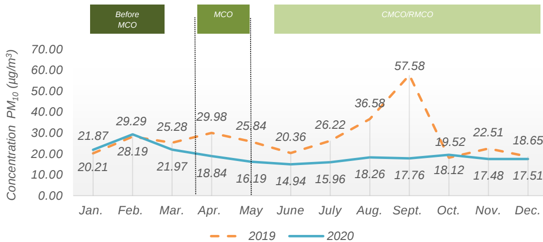
Chart 1.8: Monthly average concentration of PM_{10} in the air, Samalaju station, Sarawak, 2019 and 2020
