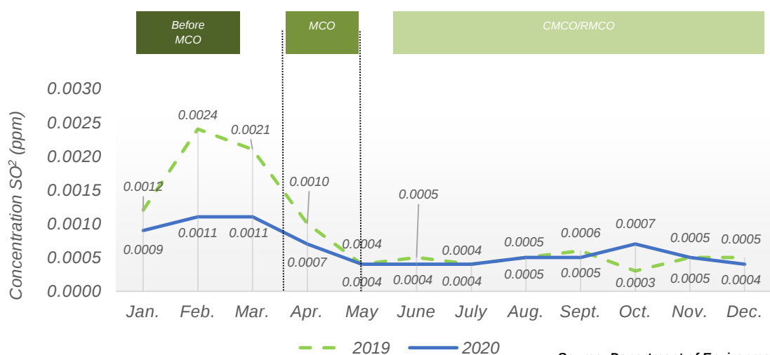
Chart 1.36: Monthly average concentration of SO 2 in the air, Samalaju station, Sarawak, 2019 and 2020
