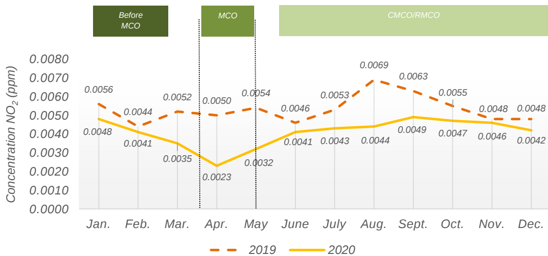
Chart 1.39: Monthly average concentration of NO 2 in the air, Kuching station, Sarawak, 2019 and 2020
