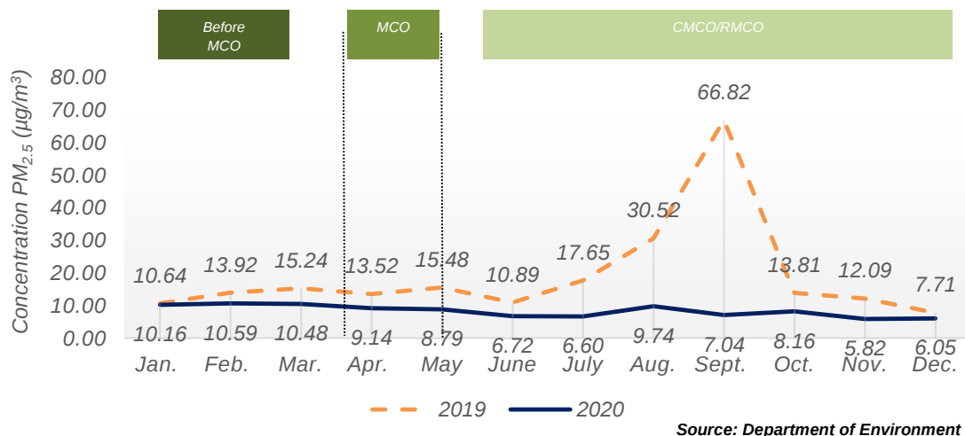
Chart 1.23: Monthly average concentration of PM 2.5 in the air, Sibul station, Sarawak, 2019 and 2020
