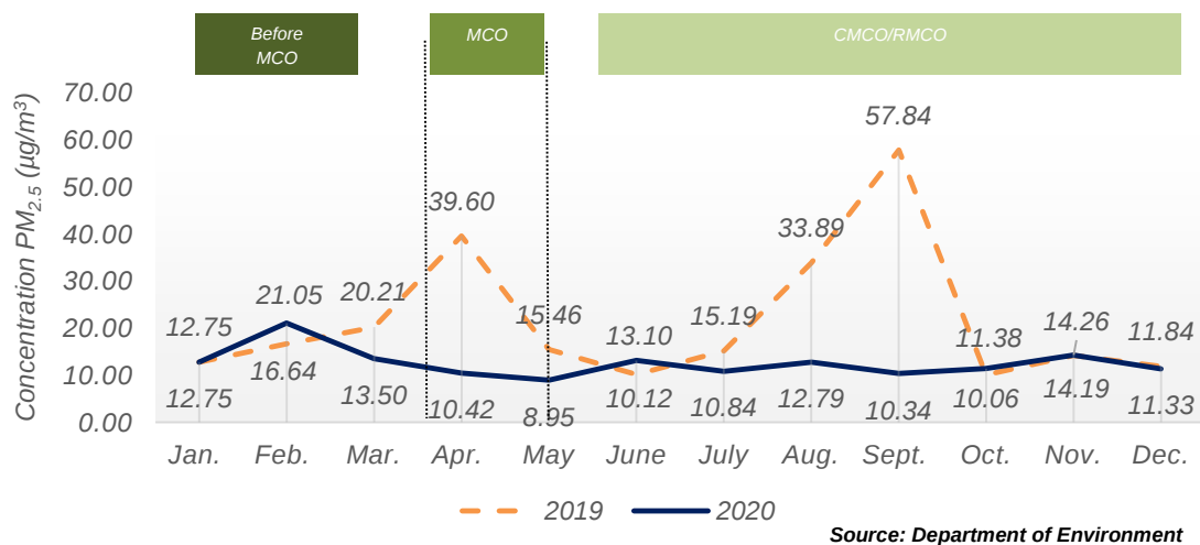
Chart 1.18: Monthly average concentration of PM 2.5 in the air, Miri station, Sarawak, 2019 and 2020
