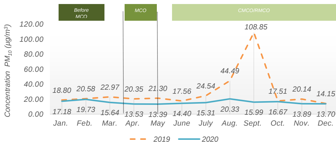
Chart 1.4: Monthly average concentration of PM 10 in the air, Kuching station, Sarawak, 2019 and 2020
