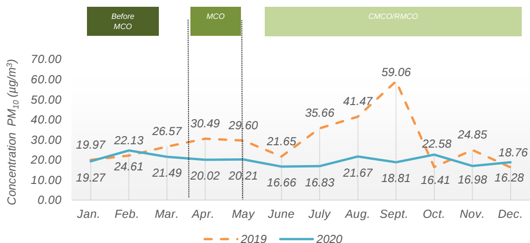
Chart 1.1: Monthly average concentration of PM_{10} in the air, Bintulu station, Sarawak, 2019 and 2020
