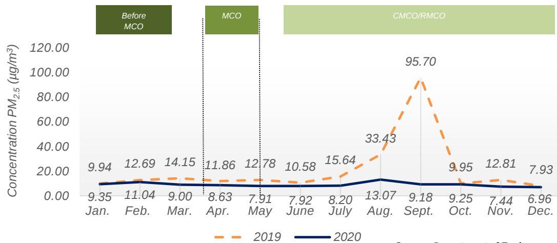
Chart 1.16: Monthly average concentration of PM 2.5 in the air, Kuching station, Sarawak, 2019 and 2020
