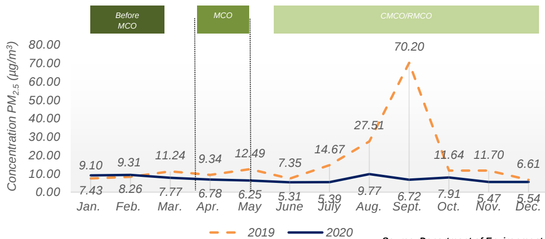
Chart 1.22: Monthly average concentration of PM 2.5 in the air, Sarikei station, Sarawak, 2019 and 2020
