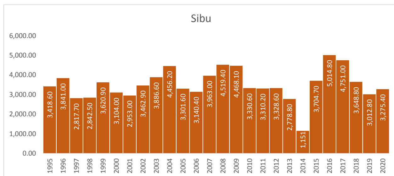
Chart 1.4: Rainfall distribution at Sibu meteorological station, Sarawak, 1995-2020
