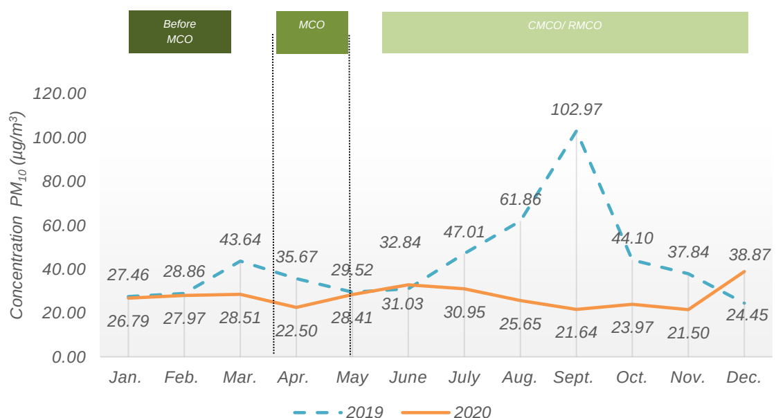
Chart 1.1: Monthly average concentration of PM_{10} in the air, Nilai station, Negeri Sembilan, 2019 and 2020
