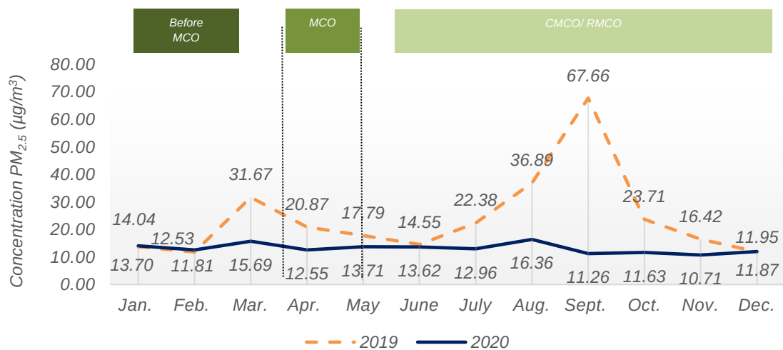
Chart 1.5: Monthly average concentration of PM 2.5 in the air, Port Dickson, Negeri Sembilan, 2019 and 2020
