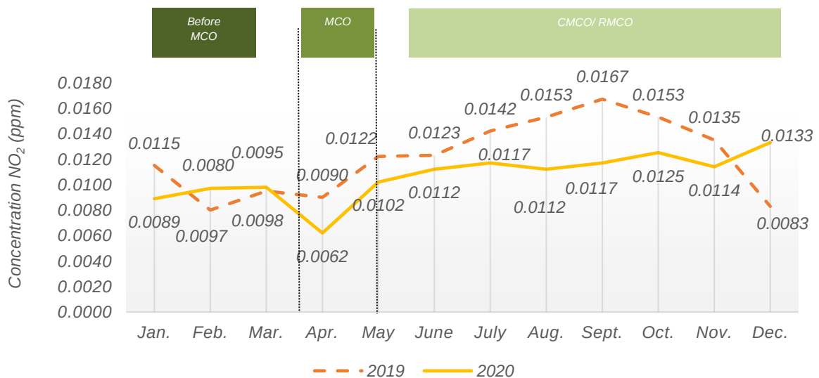
Chart 1.15: Monthly average concentration of NO 2 in the air, Nilai station, Negeri Sembilan, 2019 and 2020
