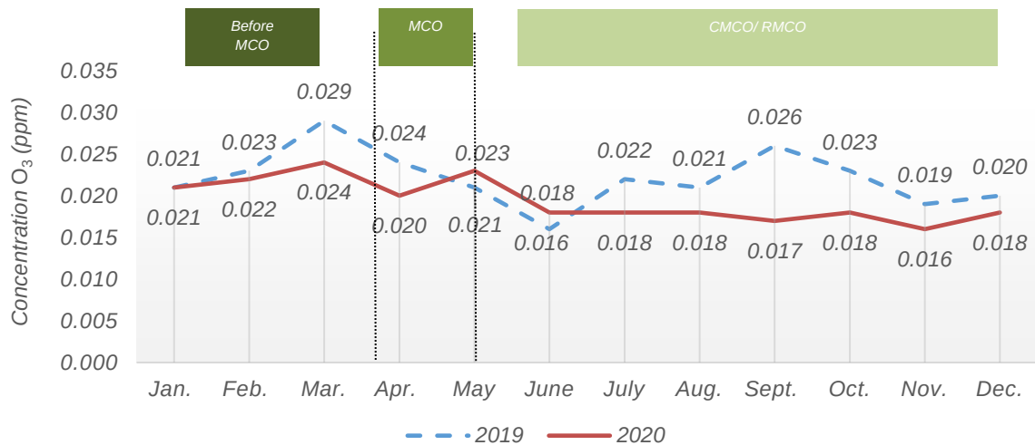
Chart 1.9: Monthly average concentration of O 3 in the air, Seremban station, Negeri Sembilan, 2019 and 2020
