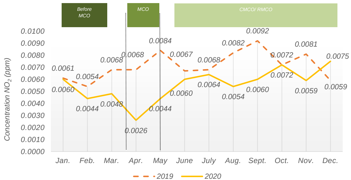
Chart 1.18: Monthly average concentration of NO 2 in the air, Seremban station, Negeri Sembilan, 2019 and 2020
