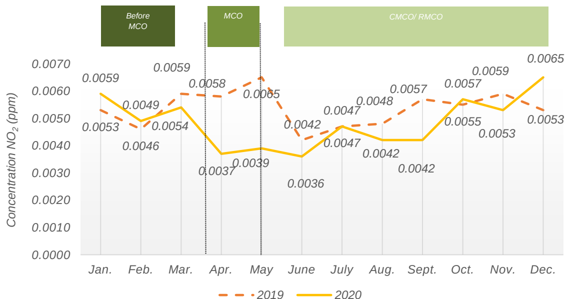
Chart 1.16: Monthly average concentration of NO 2 in the air, Port Dickson station, Negeri Sembilan, 2019 and 2020
