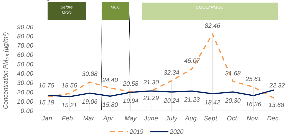
Chart 1.4: Monthly average concentration of PM 2.5 in the air, Nilai station, Negeri Sembilan, 2019 and 2020
