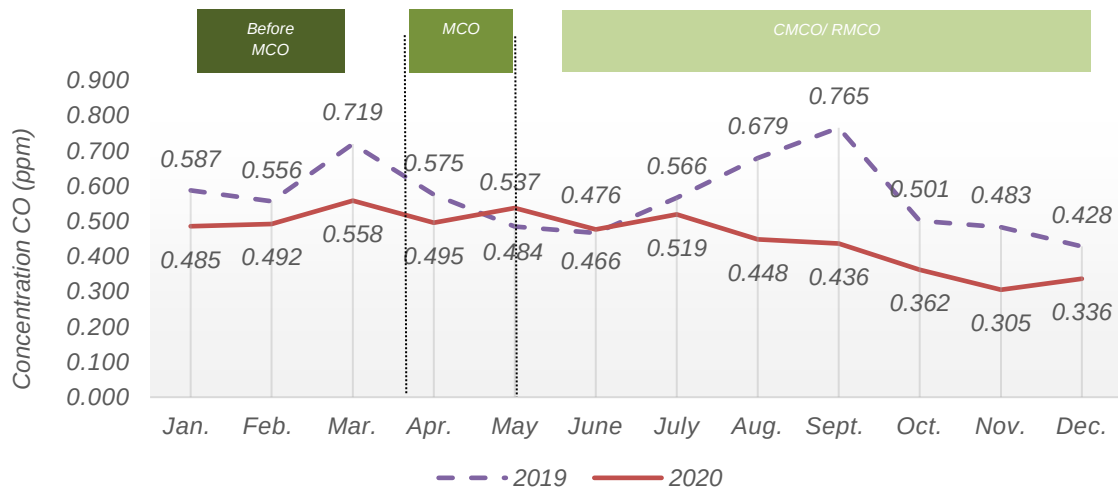
Chart 1.11: Monthly average concentration of CO in the air, Port Dickson station, Negeri Sembilan, 2019 and 2020
