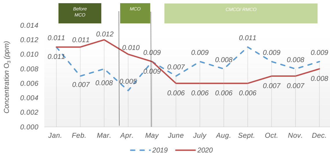
Chart 1.7: Monthly average concentration of O_3 in the air, Nilai station, Negeri Sembilan, 2019 and 2020
