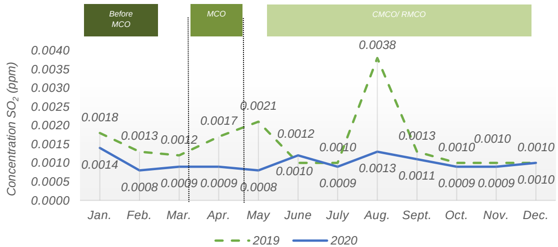
Chart 1.13: Monthly average concentration of SO 2 in the air, Nilai station, Negeri Sembilan, 2019 and 2020
