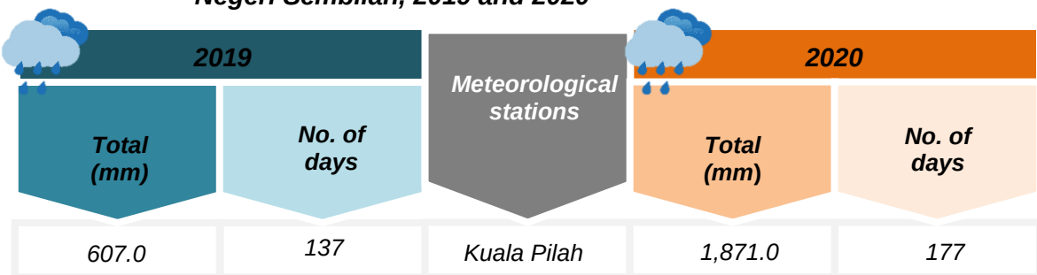
Exhibit 1.2: Total and number of rainfall days at meteorological stations, Negeri Sembilan, 2019 and 2020
