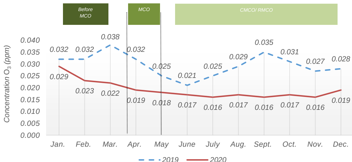
Chart 1.8: Monthly average concentration of O_3 in the air, Port Dickson station, Negeri Sembilan, 2019 and 2020
