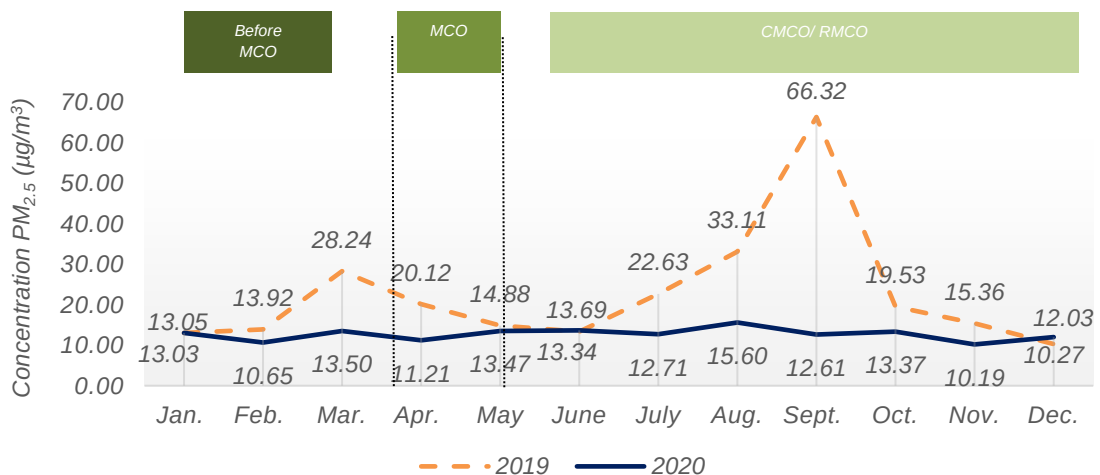
Chart 1.6: Monthly average concentration of PM 2.5 in the air, Seremban station, Negeri Sembilan, 2019 and 2020
