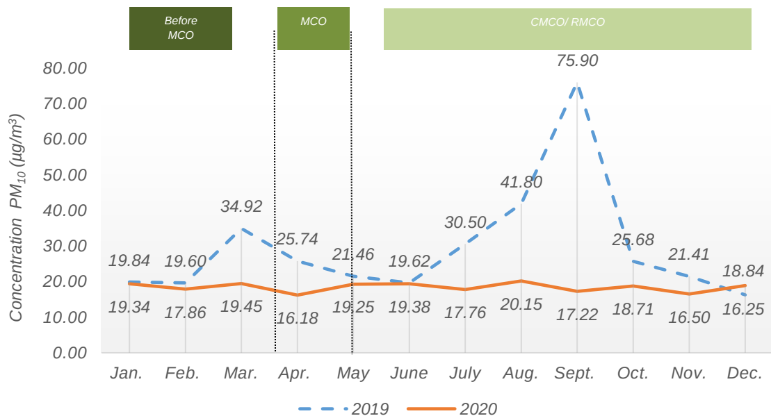
Chart 1.3: Monthly average concentration of PM_{10} in the air, Seremban station, Negeri Sembilan, 2019 and 2020
