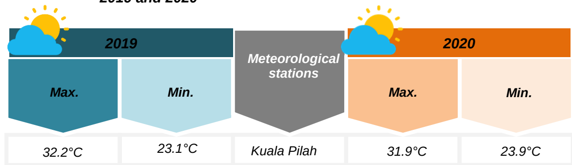
Exhibit 1.1: Mean temperature at meteorological stations, Negeri Sembilan, 2019 and 2020
