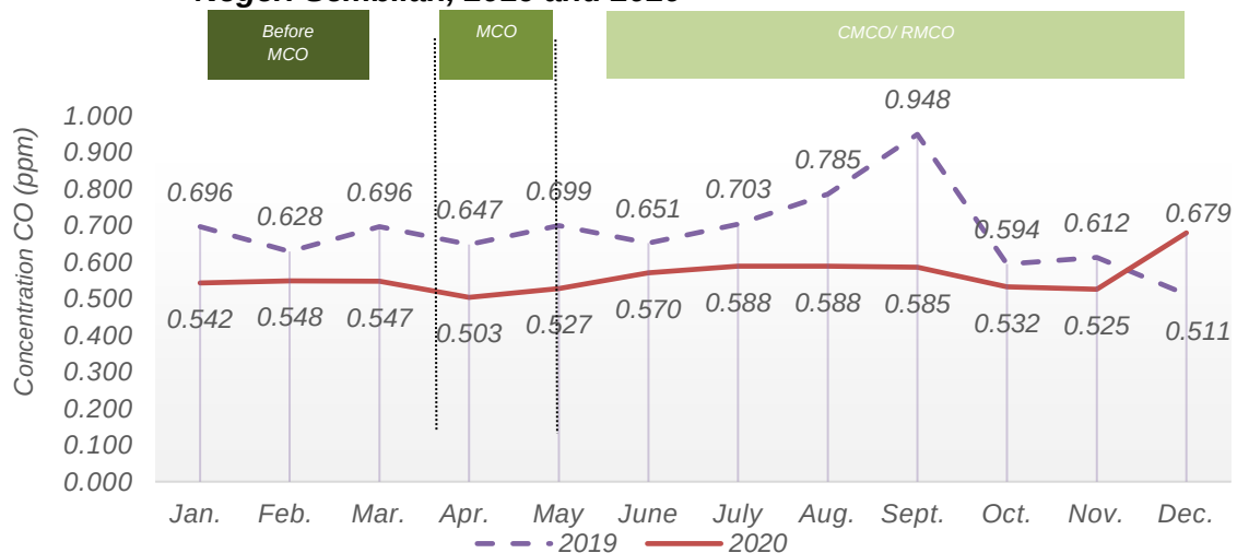
Chart 1.12: Monthly average concentration of CO in the air, Seremban station, Negeri Sembilan, 2019 and 2020
