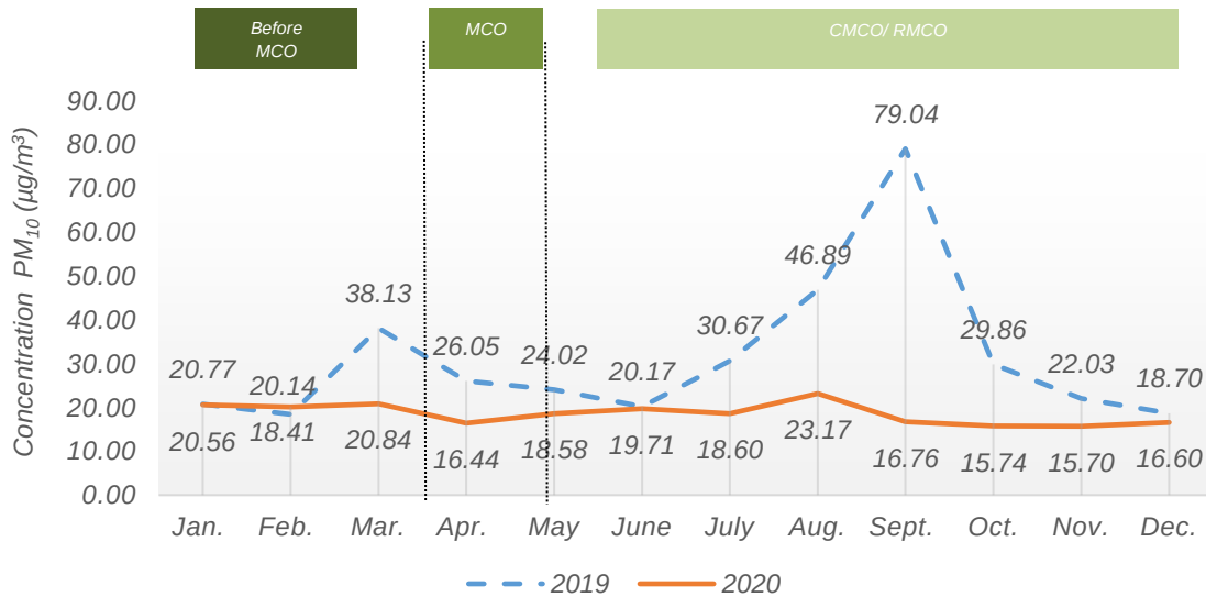
Chart 1.2: Monthly average concentration of PM_{10} in the air, Port Dickson station, Negeri Sembilan, 2019 and 2020
