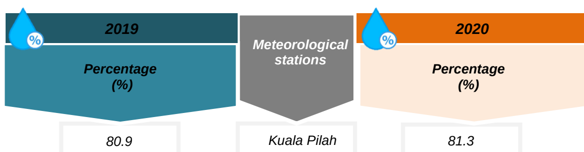
Exhibit 1.3: Mean relative humidity at meteorological stations, Negeri Sembilan, 2019 and 2020
