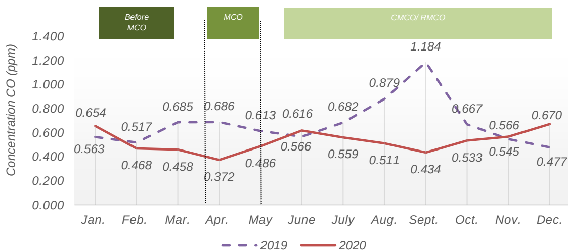
Chart 1.10: Monthly average concentration of CO in the air, Nilai station, Negeri Sembilan, 2019 and 2020
