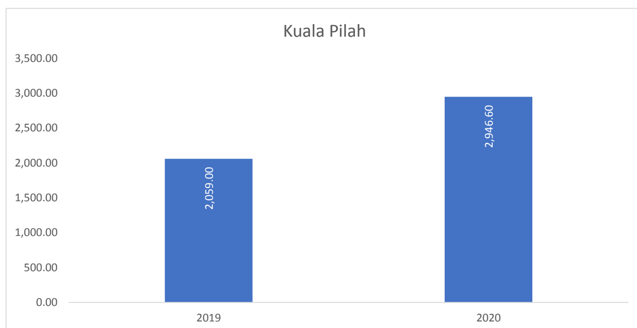
Chart 1.1: Rainfall distribution at Kuala Pilah meteorological station, Negeri Sembilan, 2019 and 2020
