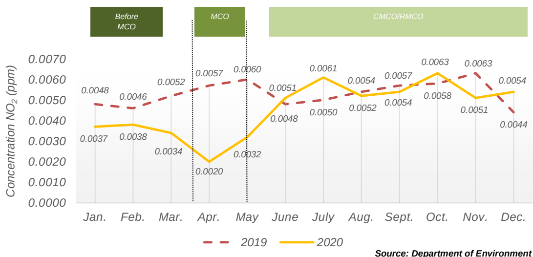
Chart 1.23: Monthly average concentration of NO 2 in the air, Kuantan station, Pahang, 2019 and 2020
