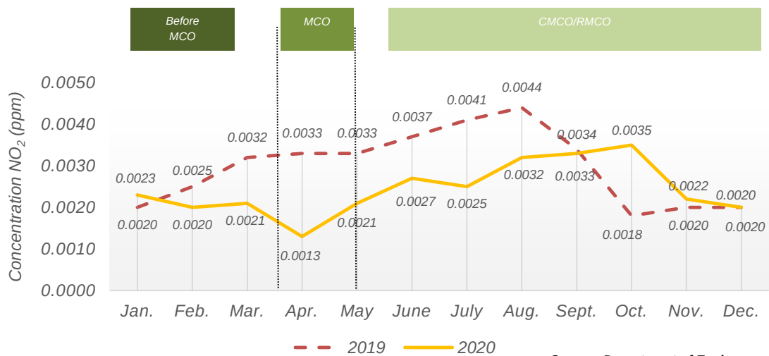
Chart 1.22: Monthly average concentration of NO 2 in the air, Jerantut station, Pahang, 2019 and 2020
