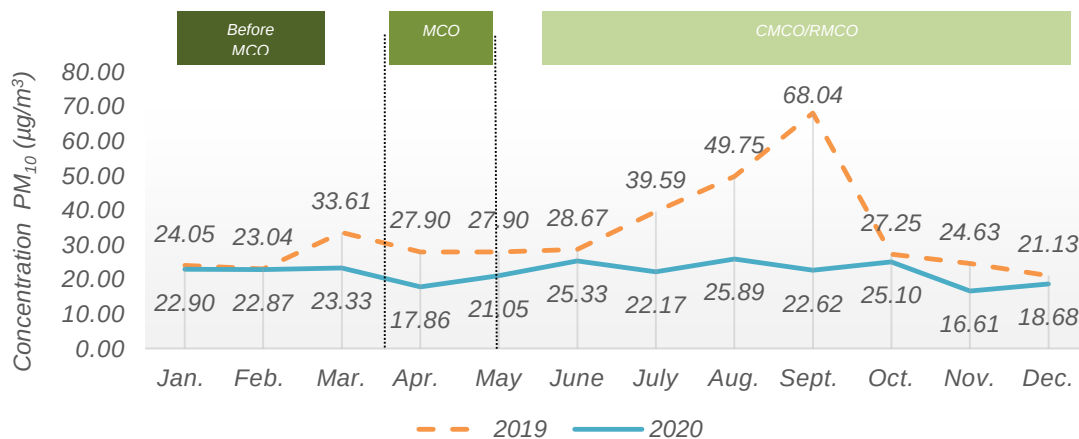
Chart 1.5: Monthly average concentration of PM_{10} in the air, Temerloh station, Pahang, 2019 and 2020
