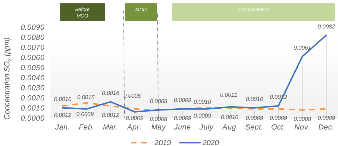
Chart 1.17: Monthly average concentration of SO 2 in the air, Balok Baru station, Pahang, 2019 and 2020
