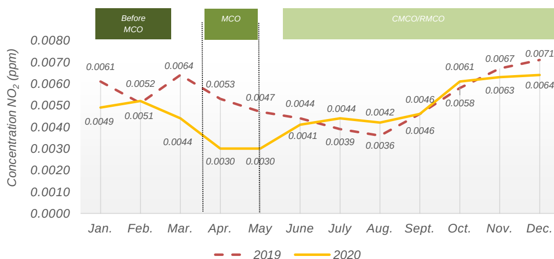
Chart 1.21: Monthly average concentration of NO 2 in the air, Balok Baru station, Pahang, 2019 and 2020
