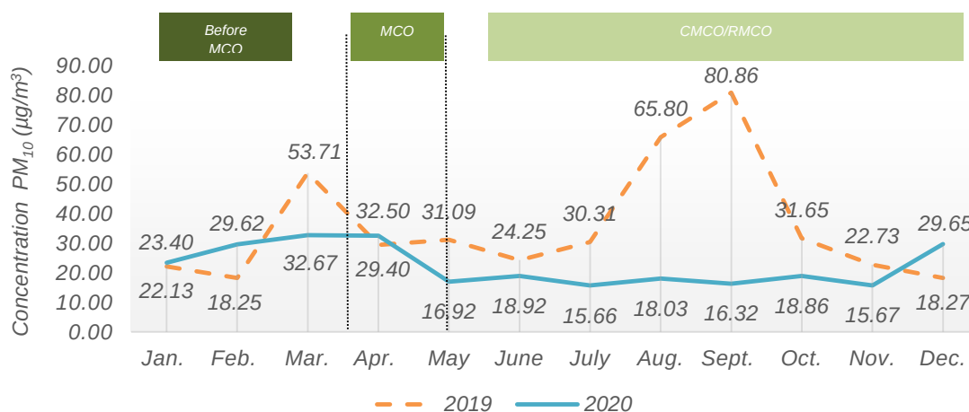
Chart 1.4: Monthly average concentration of PM_{10} in the air, Rompin station, Pahang, 2019 and 2020
