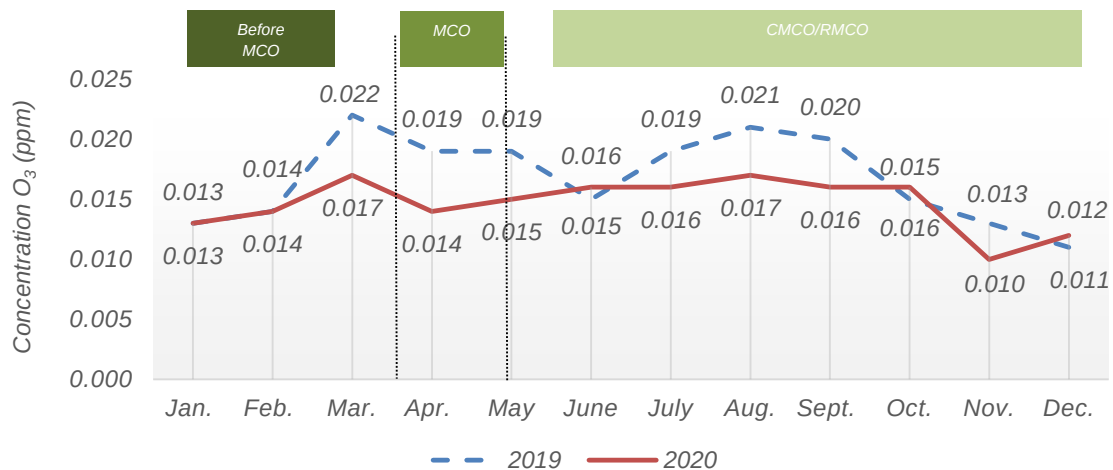
Chart 1.13: Monthly average concentration of O 3 in the air, Temerloh station, Pahang, 2019 and 2020
