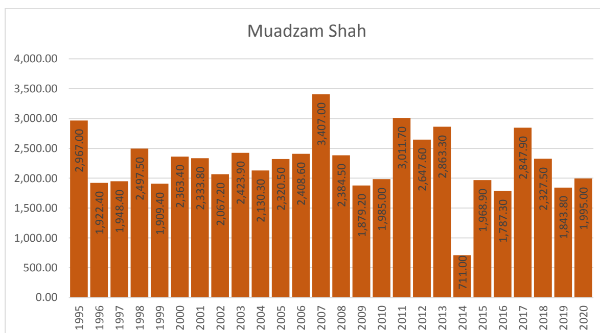
Chart 1.4: Rainfall distribution at Muadzam Shah meteorological station, Pahang, 1995-2020
