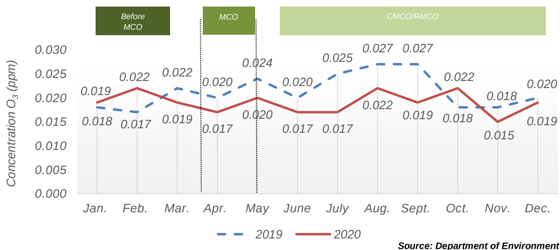
Chart 1.12: Monthly average concentration of O_3 in the air, Kuantan station, Pahang, 2019 and 2020
