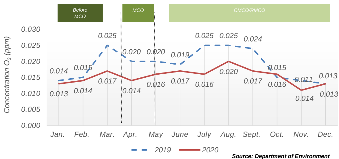
Chart 1.11: Monthly average concentration of O_3 in the air, Jerantut station, Pahang, 2019 and 2020
