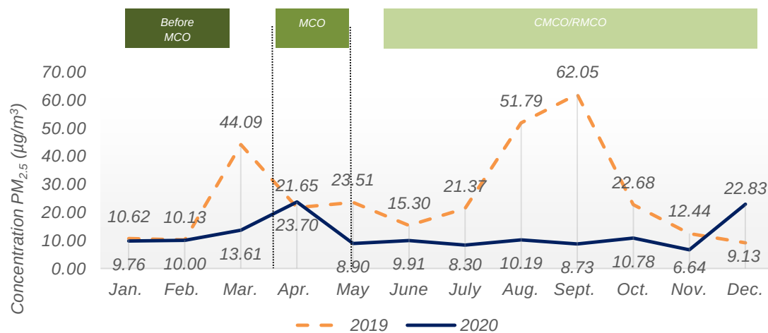
Chart 1.9: Monthly average concentration of PM 2.5 in the air, Rompin station, Pahang, 2019 and 2020
