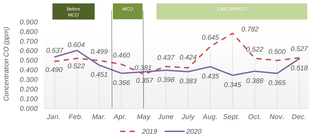
Chart 1.16: Monthly average concentration of CO in the air, Temerloh station, Pahang, 2019 and 2020
