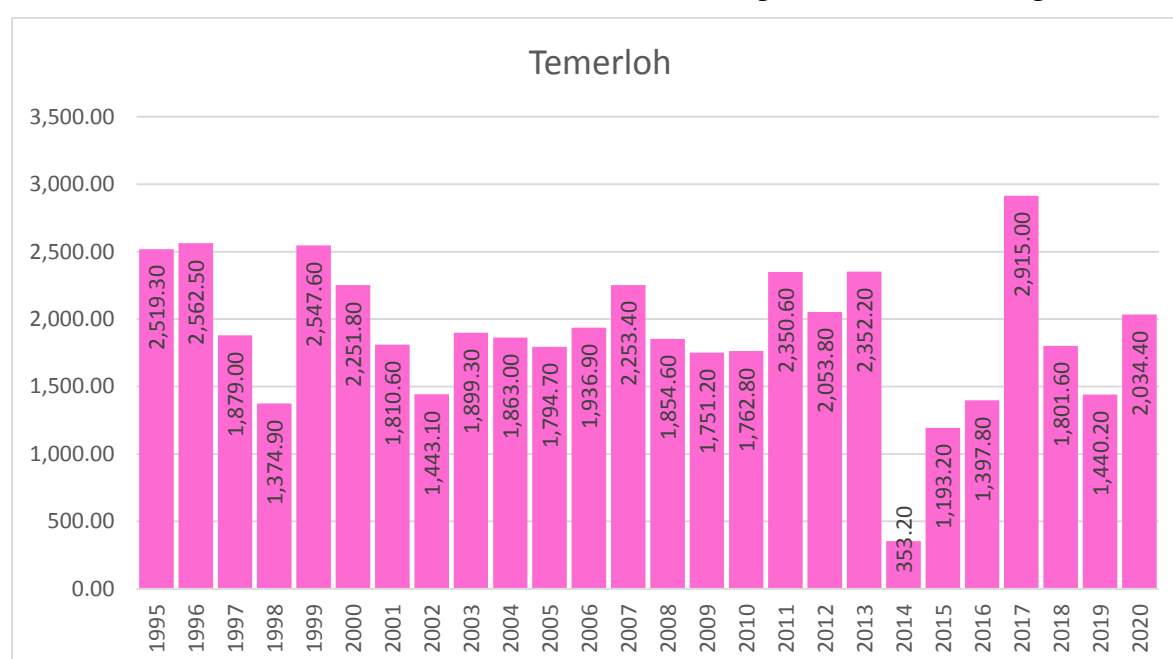
Chart 1.5: Rainfall distribution at Temerloh meteorological station, Pahang, 1995-2020
