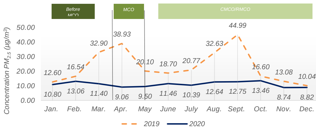
Chart 1.6: Monthly average concentration of PM_{2.5} in the air, Balok Baru station, Pahang, 2019 and 2020
