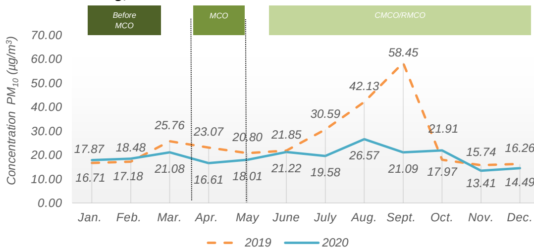
Chart 1.2: Monthly average concentration of PM_{10} in the air, Jerantut station, Pahang, 2019 and 2020
