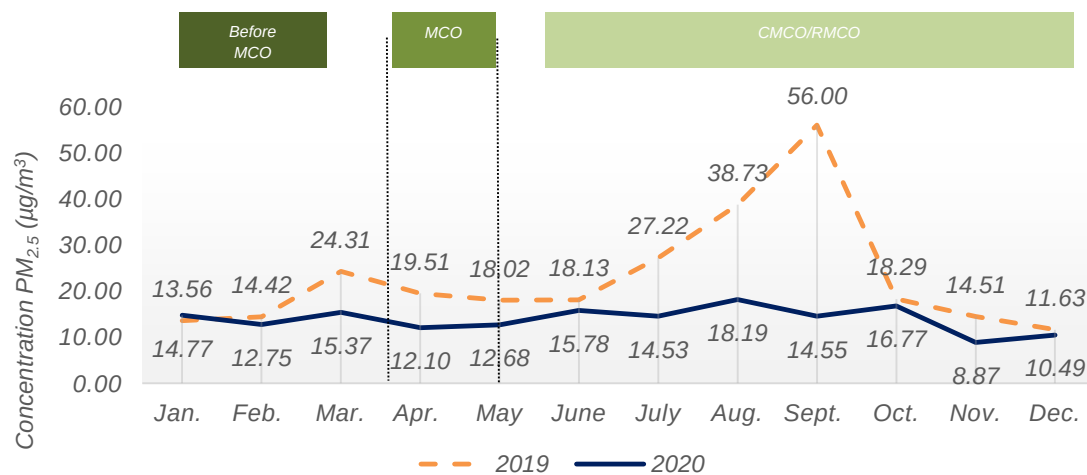
Chart 1.10: Monthly average concentration of PM 2.5 in the air, Temerloh station, Pahang, 2019 and 2020
