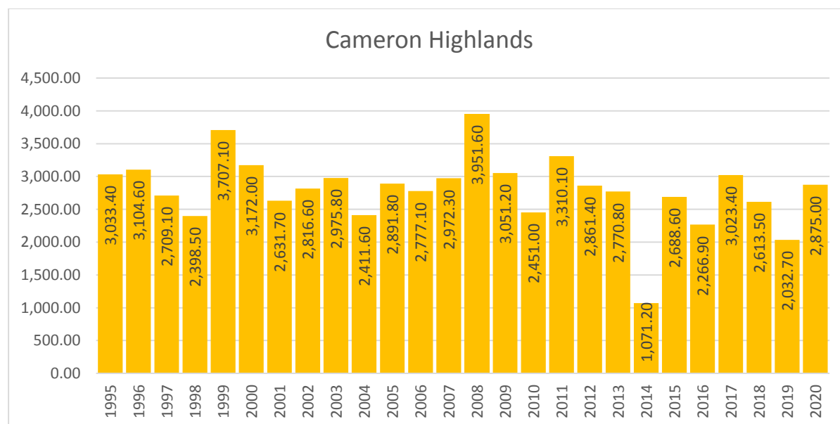
Chart 1.2: Rainfall distribution at Cameron Highlands meteorological station, Pahang, 1995-2020
