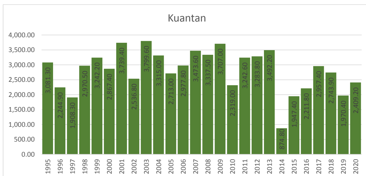
Chart 1.3: Rainfall distribution at Kuantan meteorological station, Pahang, 1995-2020
