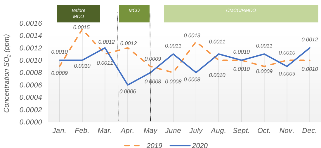
Chart 1.19: Monthly average concentration of SO 2 in the air, Kuantan station, Pahang, 2019 and 2020
