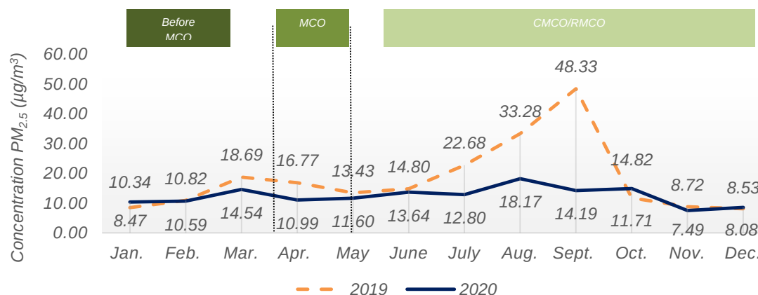
Chart 1.7: Monthly average concentration of PM_{2.5} in the air, Jerantut station, Pahang, 2019 and 2020
