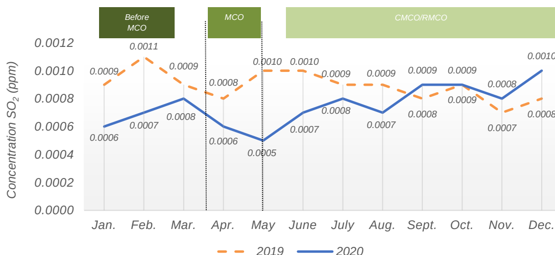
Chart 1.20: Monthly average concentration of SO 2 in the air, Temerloh station, Pahang, 2019 and 2020
