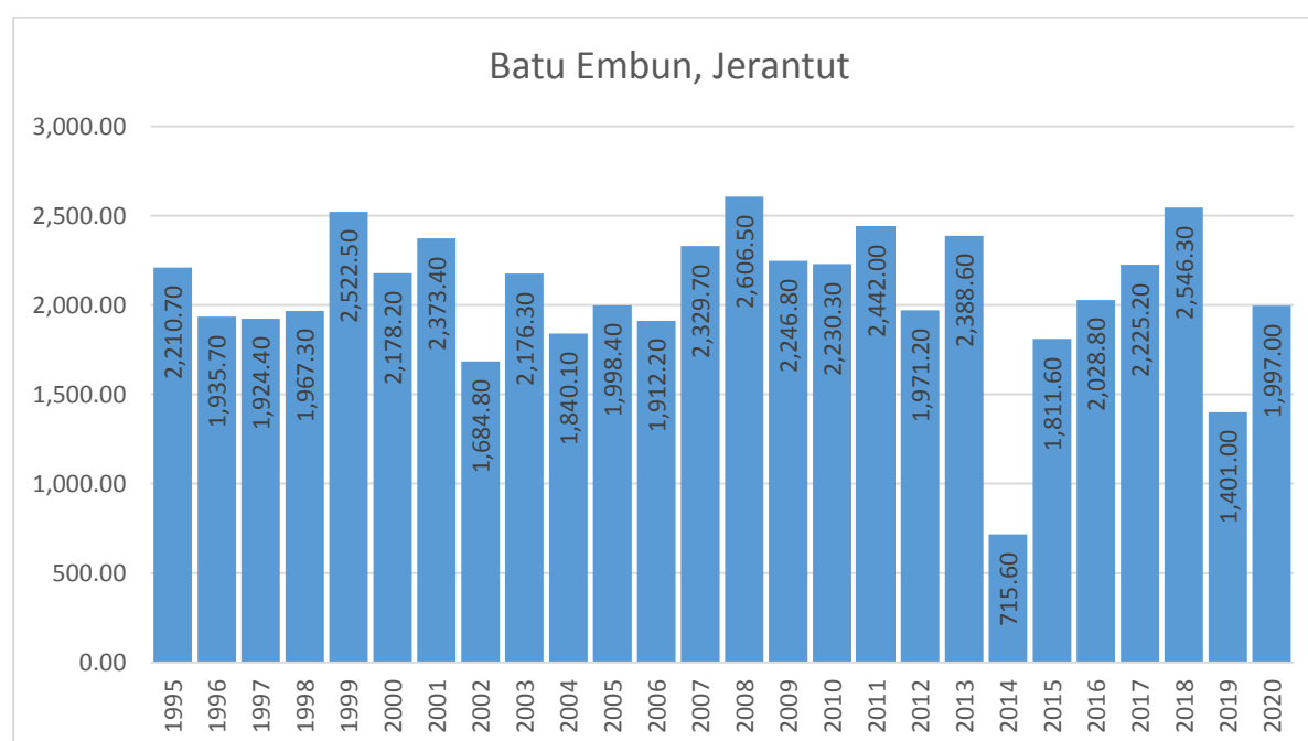
Chart 1.1: Rainfall distribution at Batu Embun, Jerantut meteorological station, Pahang, 1995-2020
