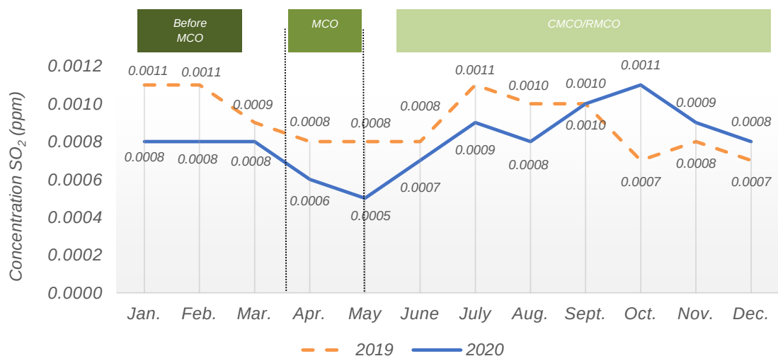
Chart 1.18: Monthly average concentration of SO 2 in the air, Jerantut station, Pahang, 2019 and 2020
