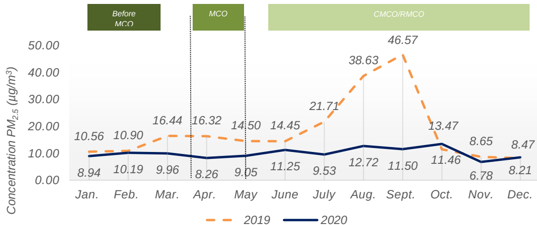
Chart 1.8: Monthly average concentration of PM 2.5 in the air, Kuantan station, Pahang, 2019 and 2020
