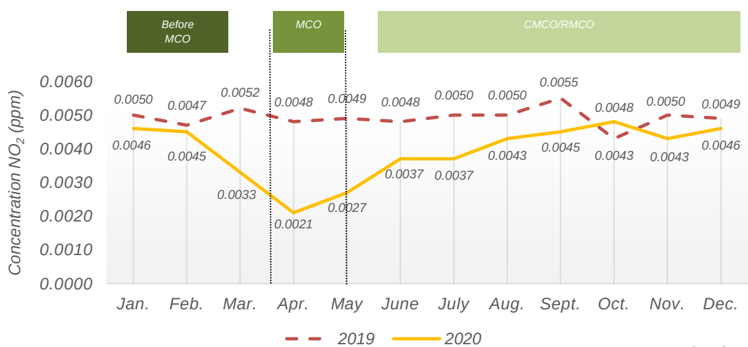
Chart 1.24: Monthly average concentration of NO 2 in the air, Temerloh station, Pahang, 2019 and 2020
