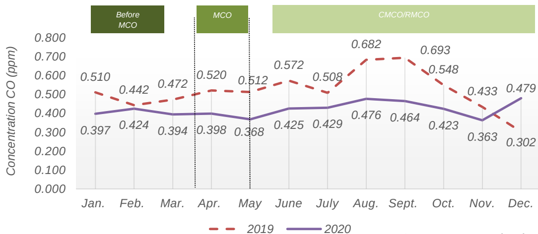
Chart 1.15: Monthly average concentration of CO in the air, Kuantan station, Pahang, 2019 and 2020
