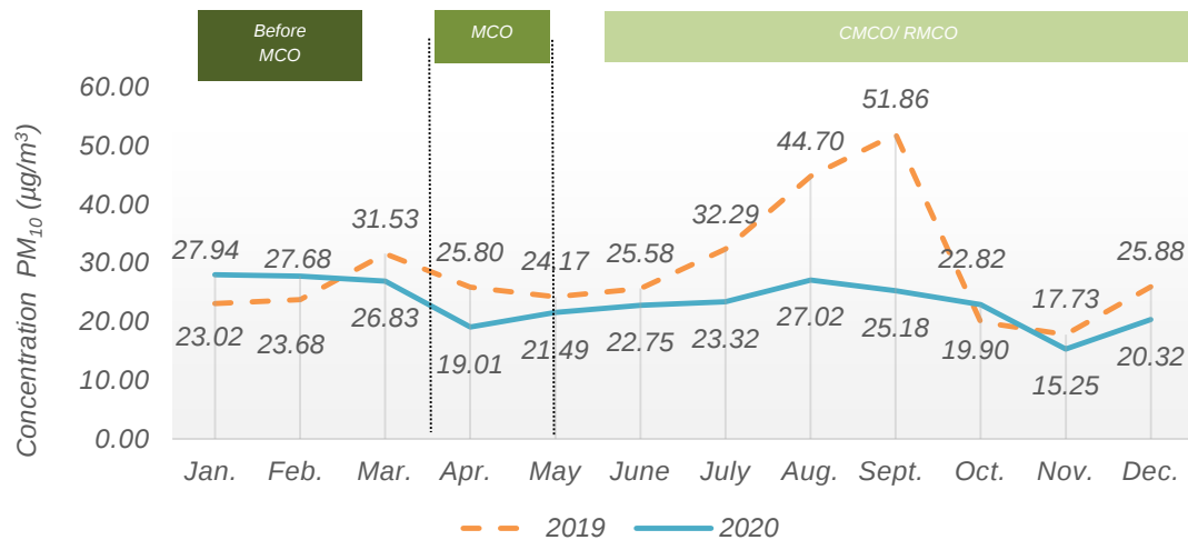
Chart 1.3: Monthly average concentration of PM 10 in the air, Kuala Terengganu station, Terengganu, 2019 and 2020
