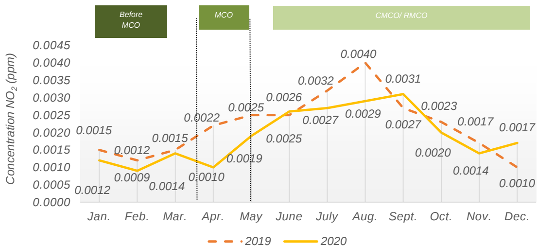
Chart 1.20: Monthly average concentration of NO 2 in the air, Paka station, Terengganu, 2019 and 2020
