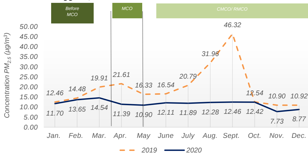
Chart 1.6: Monthly average concentration of PM_{2.5} in the air, Kemaman station, Terengganu, 2019 and 2020
