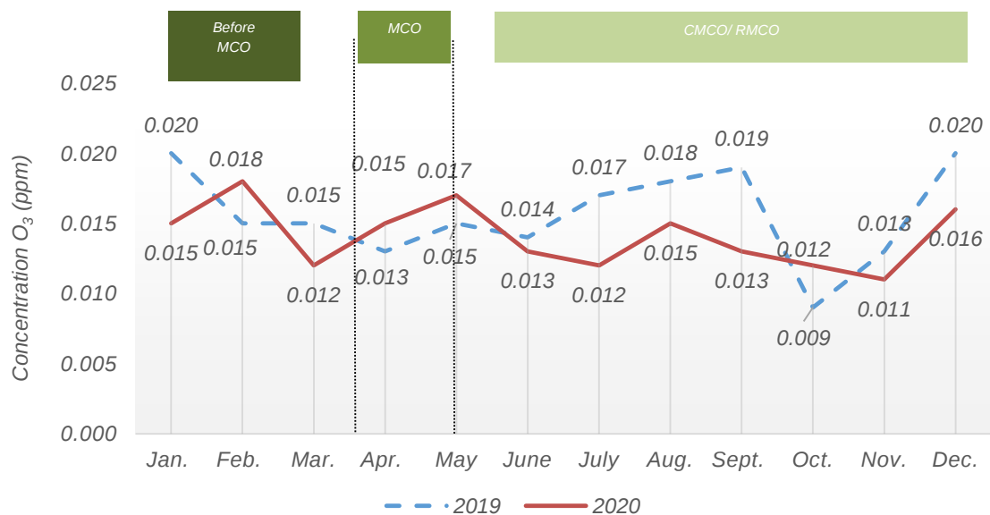
Chart 1.12: Monthly average concentration of O 3 in the air, Kuala Terengganu station, Terengganu, 2019 and 2020
