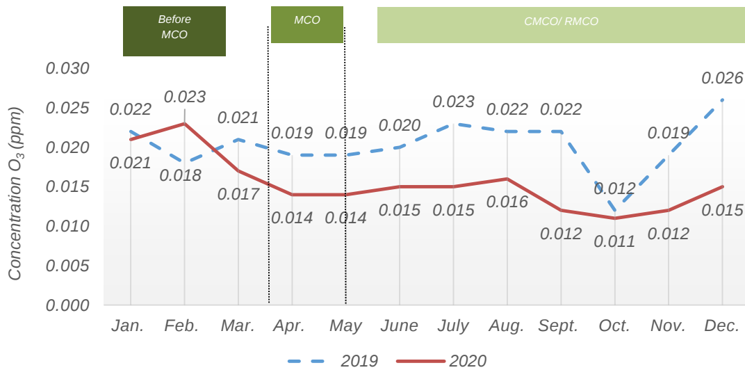
Chart 1.9: Monthly average concentration of O 3 in the air, Besut station, Terengganu, 2019 and 2020
