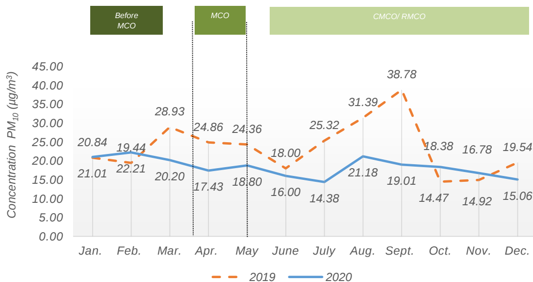
Chart 1.1: Monthly average concentration of PM_{10} in the air, Besut station, Terengganu, 2019 and 2020
