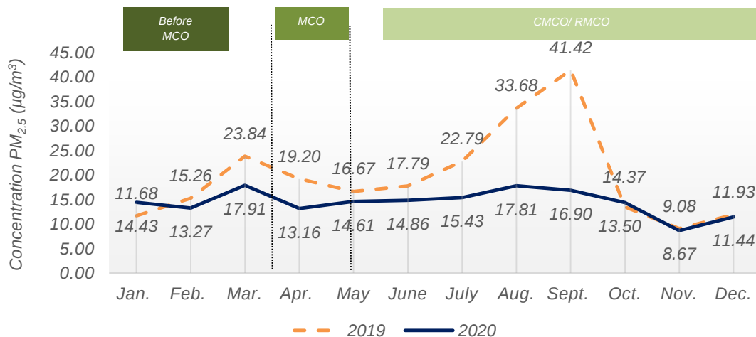
Chart 1.7: Monthly average concentration of PM_{2.5} in the air, Kuala Terengganu station, Terengganu, 2019 and 2020
