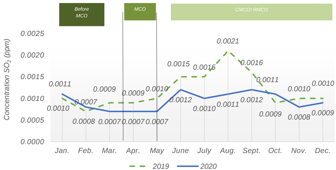
Chart 1.16: Monthly average concentration of SO 2 in the air, Paka station, Terengganu, 2019 and 2020
