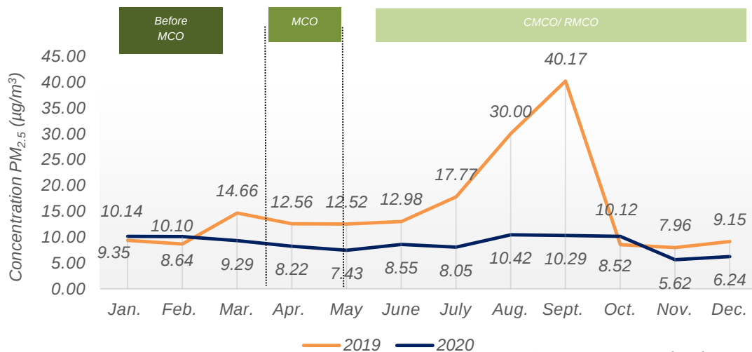
Chart 1.8: Monthly average concentration of PM_{2.5} in the air, Paka station, Terengganu, 2019 and 2020
