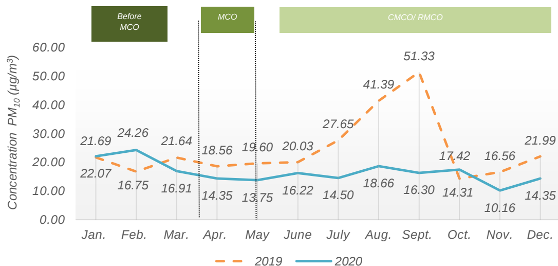
Chart 1.4: Monthly average concentration of PM 10 in the air, Paka station, Terengganu, 2019 and 2020
