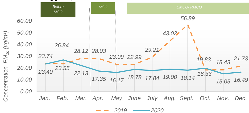
Chart 1.2: Monthly average concentration of PM 10 in the air, Kemaman station, Terengganu, 2019 and 2020
