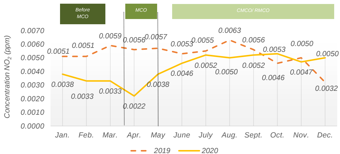
Chart 1.19: Monthly average concentration of NO 2 in the air, Kuala Terengganu station, Terengganu, 2019 and 2020
