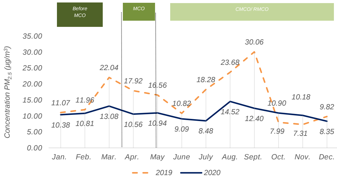
Chart 1.5: Monthly average concentration of PM_{2.5} in the air, Besut station, Terengganu, 2019 and 2020
