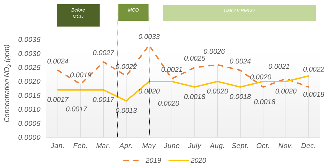
Chart 1.17: Monthly average concentration of NO 2 in the air, Besut station, Terengganu, 2019 and 2020
