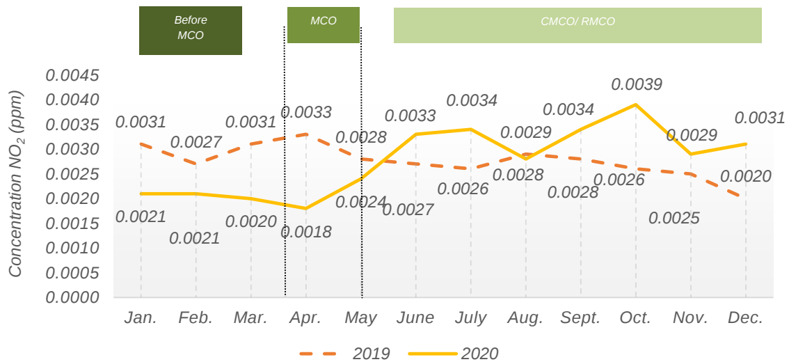
Chart 1.18: Monthly average concentration of NO 2 in the air, Kemaman station, Terengganu, 2019 and 2020
