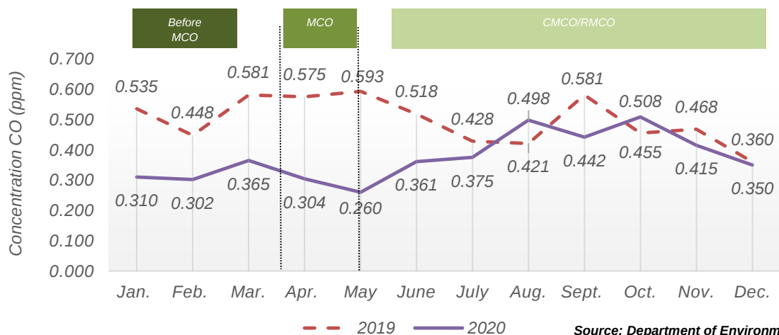
Chart 1.13: Monthly average concentration of CO in the air, Langkawi station, Kedah, 2019 and 2020
