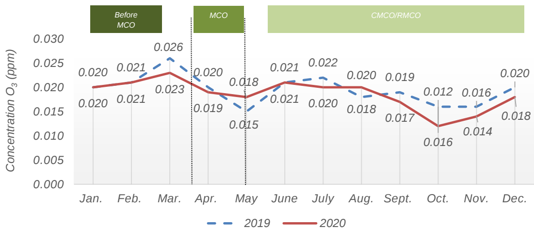
Chart 1.11: Monthly average concentration of O 3 in the air, Sungai Petani station, Kedah, 2019 and 2020
