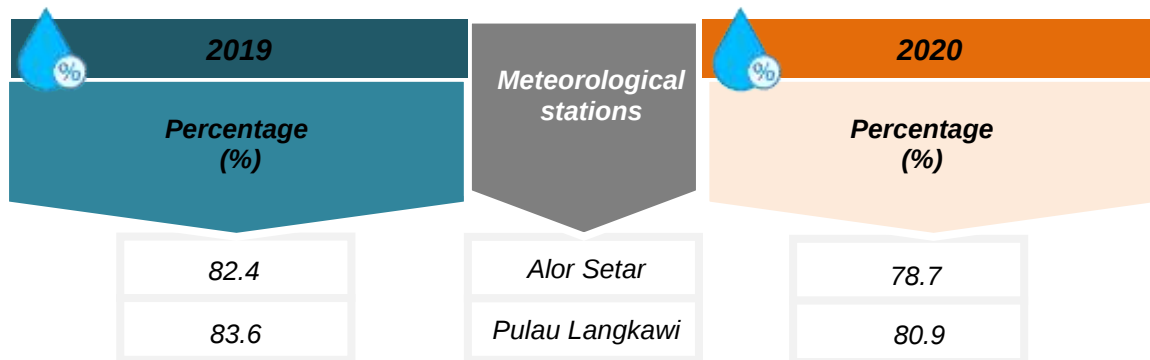
Exhibit 1.3: Mean relative humidity at meteorological stations, Kedah, 2019 and 2020
