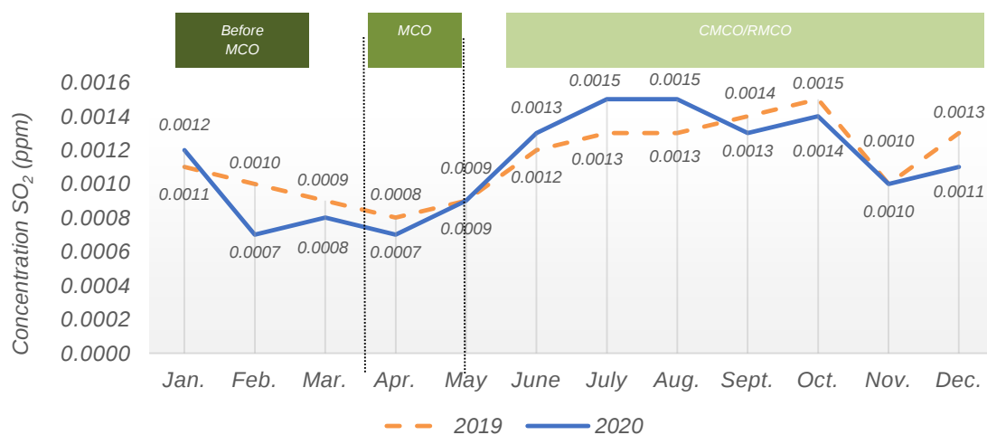
Chart 1.18: Monthly average concentration of SO 2 in the air, Sungai Petani station, Kedah, 2019 and 2020
