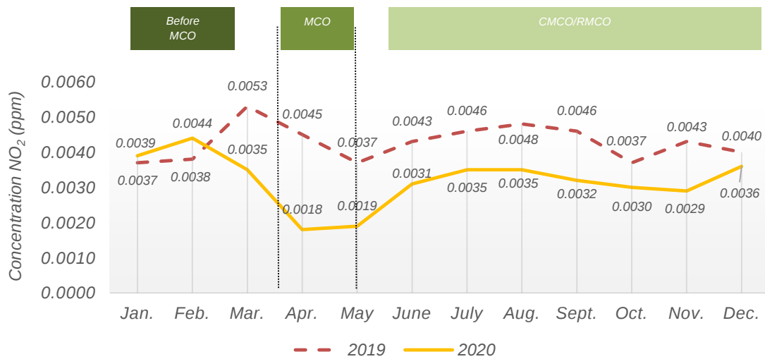
Chart 1.21: Monthly average concentration of NO 2 in the air, Langkawi station, Kedah, 2019 and 2020
