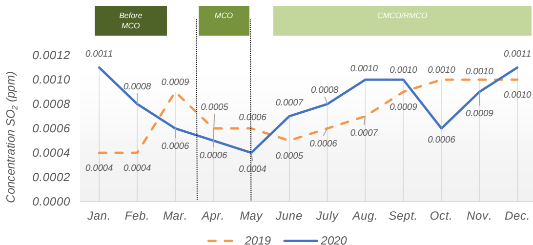
Chart 1.15: Monthly average concentration of SO 2 in the air, Alor Setar station, Kedah, 2019 and 2020
