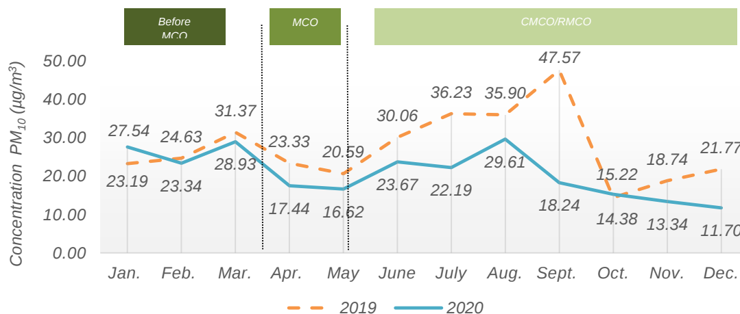
Chart 1.4: Monthly average concentration of PM 10 in the air, Sungai Petani station, Kedah, 2019 and 2020
