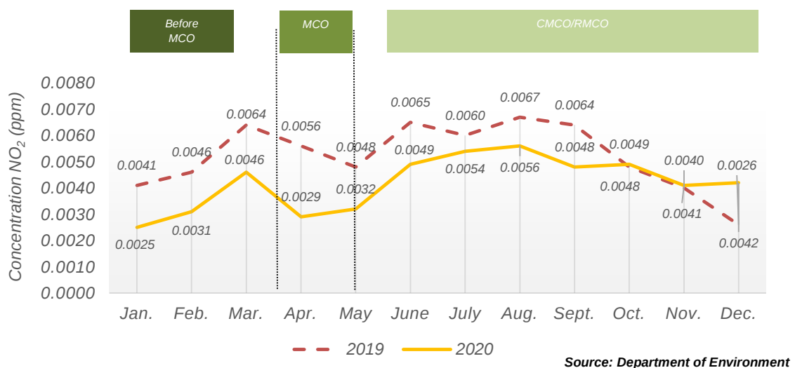
Chart 1.19: Monthly average concentration of NO 2 in the air, Alor Setar station, Kedah, 2019 and 2020
