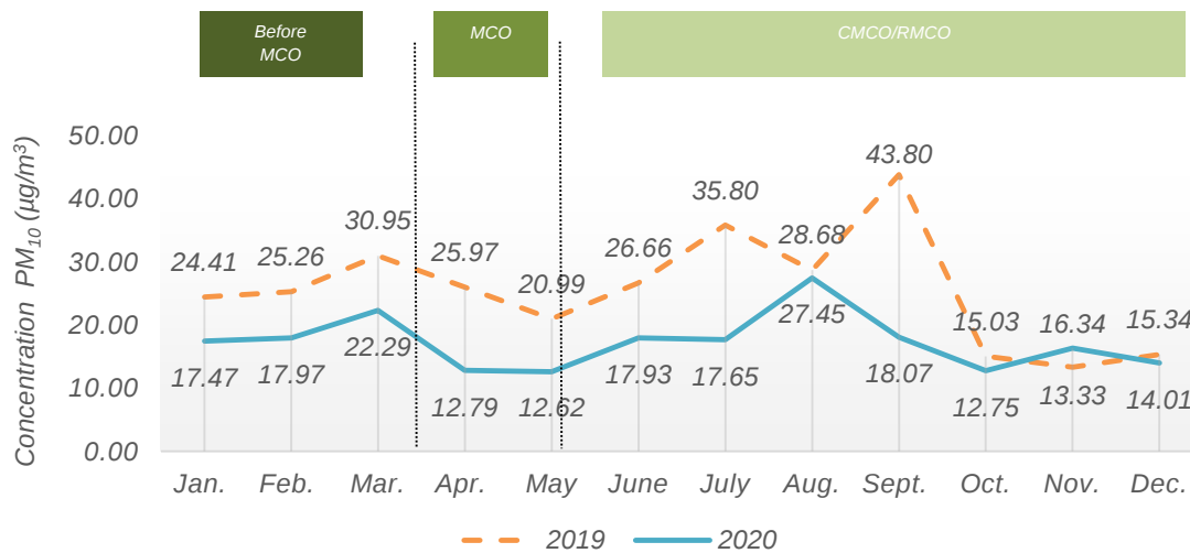
Chart 1.2: Monthly average concentration of PM 10 in the air, Kulim station, Kedah, 2019 and 2020
