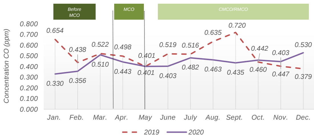
Chart 1.12: Monthly average concentration of CO in the air, Alor Setar station, Kedah, 2019 and 2020
