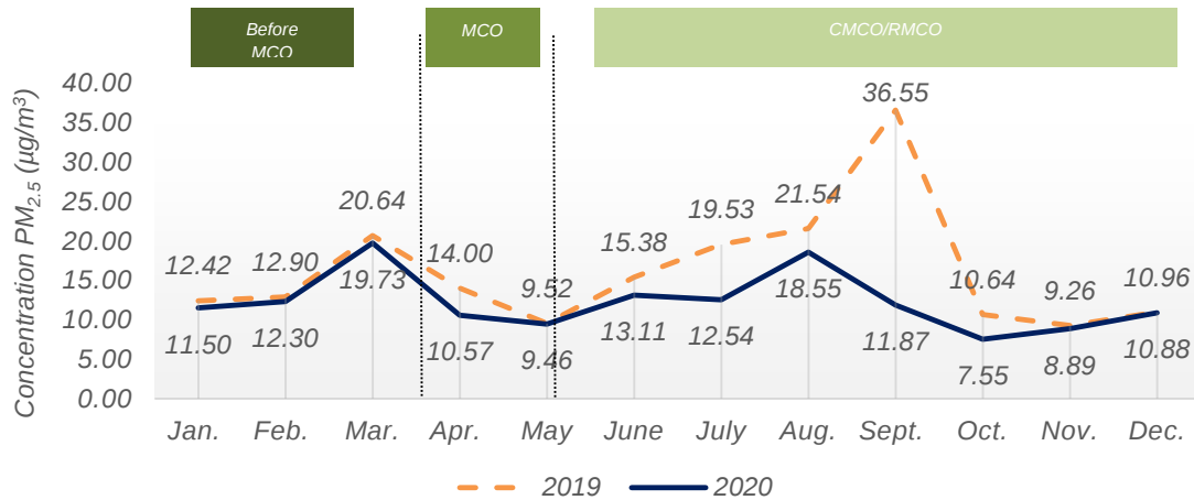
Chart 1.5: Monthly average concentration of PM_{2.5} in the air, Alor Setar station, Kedah, 2019 and 2020
