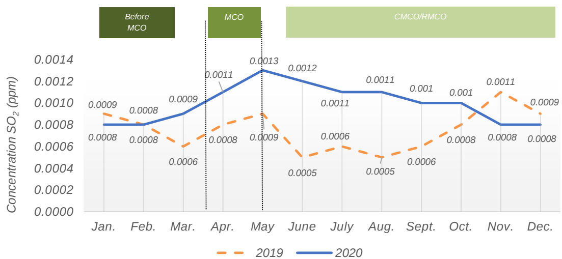
Chart 1.17: Monthly average concentration of SO 2 in the air, Langkawi station, Kedah, 2019 and 2020
