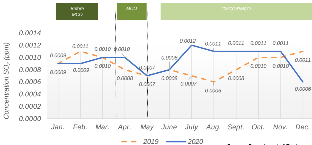
Chart 1.16: Monthly average concentration of SO 2 in the air, Kulim station, Kedah, 2019 and 2020
