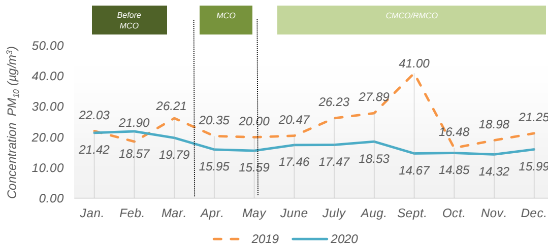
Chart 1.3: Monthly average concentration of PM 10 in the air, Langkawi station, Kedah, 2019 and 2020
