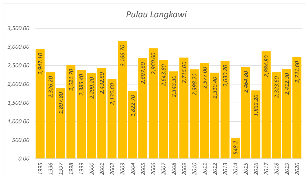
Chart 1.2: Rainfall distribution at Pulau Langkawi meteorological station, Kedah, 1995-2020
