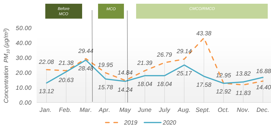
Chart 1.1: Monthly average concentration of PM_{10} in the air, Alor Setar station, Kedah, 2019 and 2020
