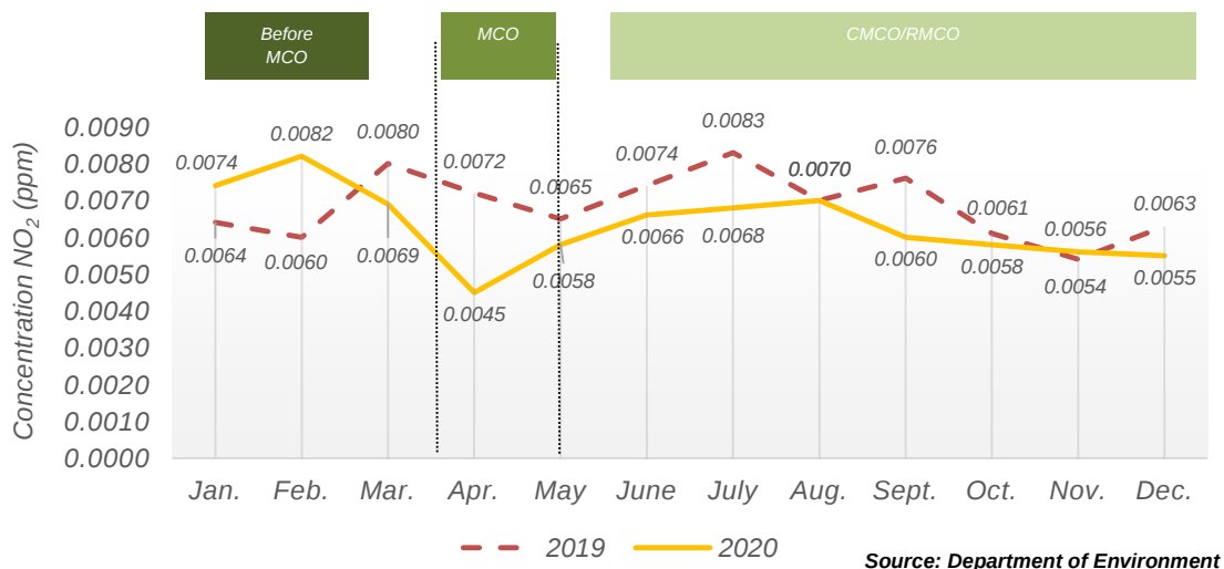
Chart 1.20: Monthly average concentration of NO 2 in the air, Kulim station, Kedah, 2019 and 2020
