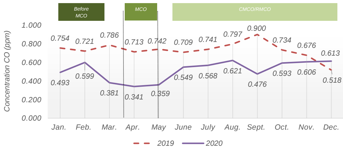
Chart 1.14: Monthly average concentration of CO in the air, Sungai Petani station, Kedah, 2019 and 2020
