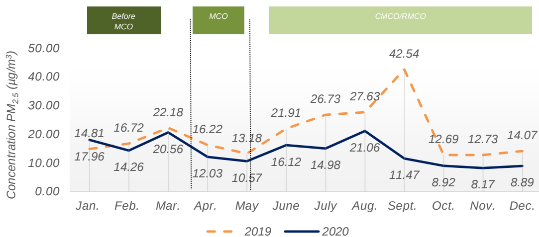
Chart 1.8: Monthly average concentration of PM 2.5 in the air, Sungai Petani station, Kedah, 2019 and 2020
