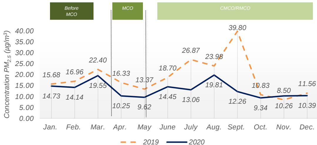
Chart 1.6: Monthly average concentration of PM_{2.5} in the air, Kulim station, Kedah, 2019 and 2020
