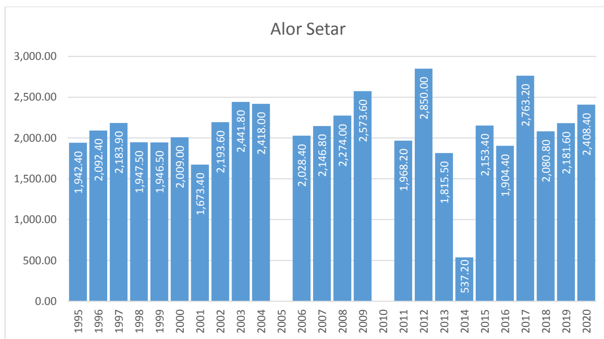
Carta1.1: Taburan hujan di stesen meteorologi Alor Setar, Kedah, 1995-2020
