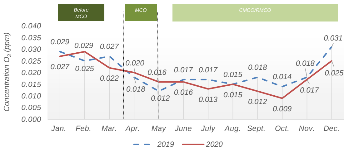
Chart 1.10: Monthly average concentration of O 3 in the air, Langkawi station, Kedah, 2019 and 2020
