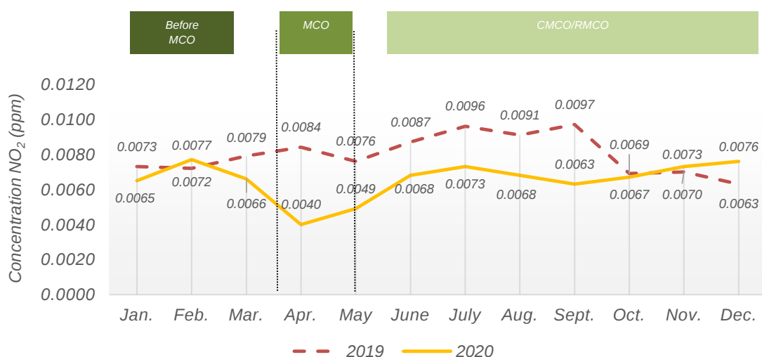
Chart 1.22: Monthly average concentration of NO 2 in the air, Sungai Petani station, Kedah, 2019 and 2020
