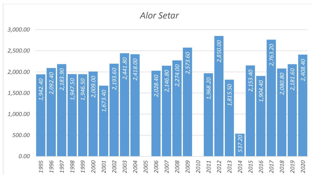
Chart 1.1: Rainfall distribution at Alor Setar meteorological station, Kedah, 1995-2020
