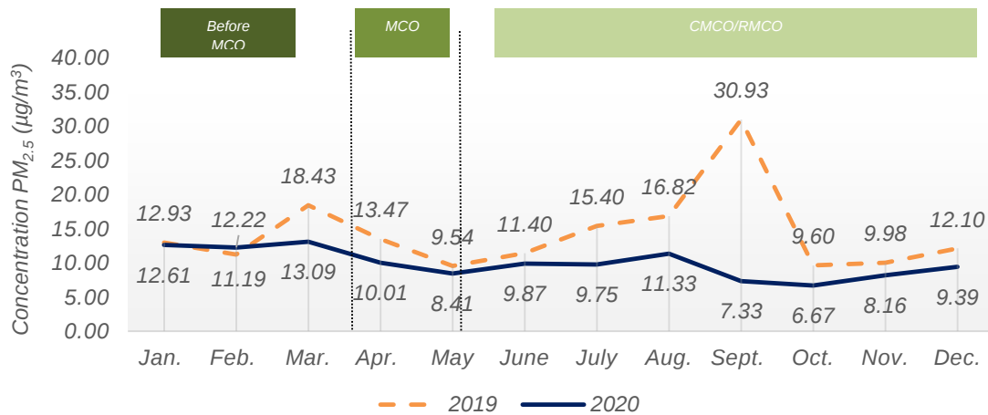
Chart 1.7: Monthly average concentration of PM 2.5 in the air, Langkawi station, Kedah, 2019 and 2020
