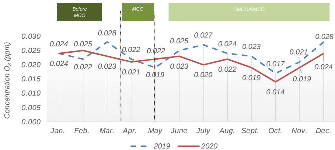
Chart 1.9: Monthly average concentration of O 3 in the air, Alor Setar station, Kedah, 2019 and 2020
