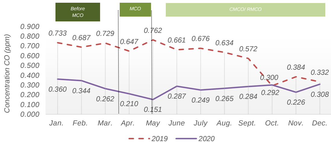
Chart 1.16: Monthly average concentration of CO in the air, Taiping station, Perak, 2019 and 2020
