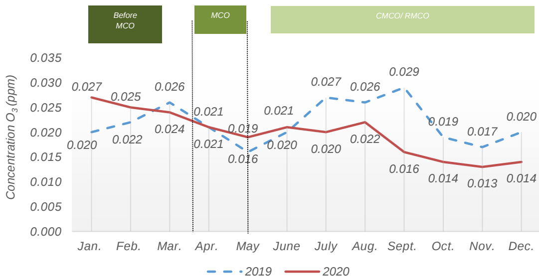
Chart 1.11: Monthly average concentration of O 3 in the air, Pegoh, Ipoh station, Perak, 2019 and 2020
