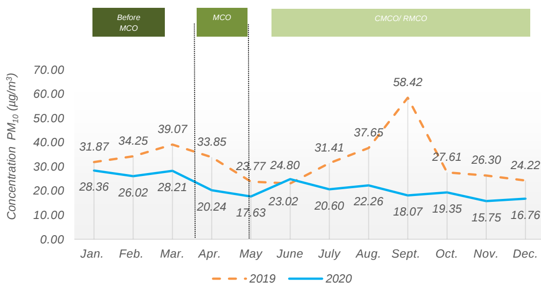
Chart 1.1: Monthly average concentration of PM_{10} in the air, Pegoh, Ipoh station, Perak, 2019 and 2020
