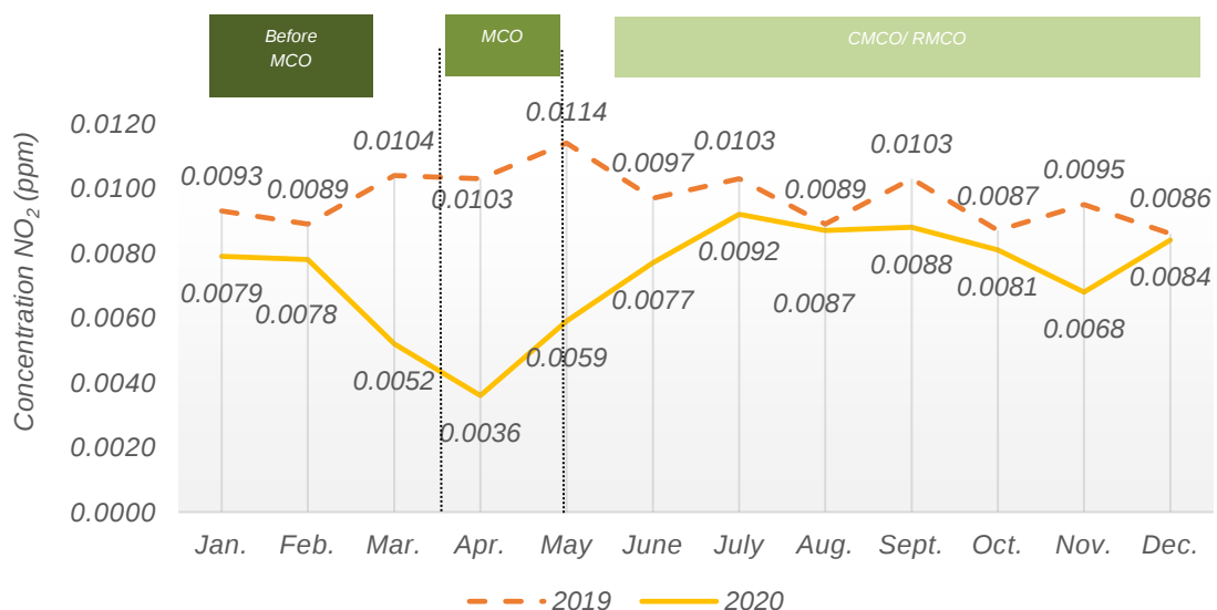
Chart 1.23: Monthly average concentration of NO 2 in the air, Pegoh, Ipoh station, Perak, 2019 and 2020
