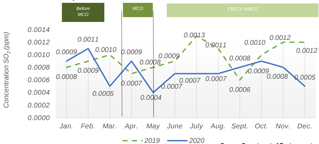
Chart 1.19: Monthly average concentration of SO 2 in the air, Pegoh, Ipoh station, Perak, 2019 and 2020
