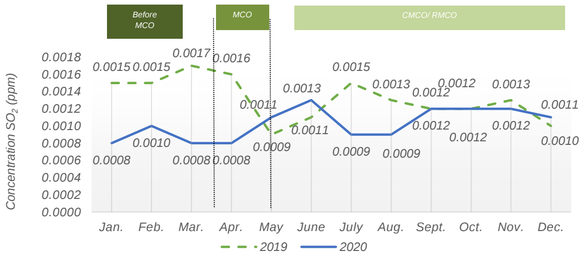
Chart 1.22: Monthly average concentration of SO 2 in the air, Tasek, Ipoh station, Perak, 2019 and 2020
