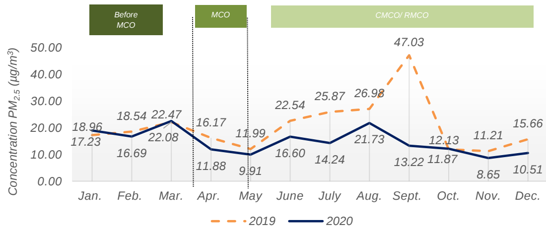
Chart 1.8: Monthly average concentration of PM 2.5 in the air, Taiping station, Perak, 2019 and 2020
