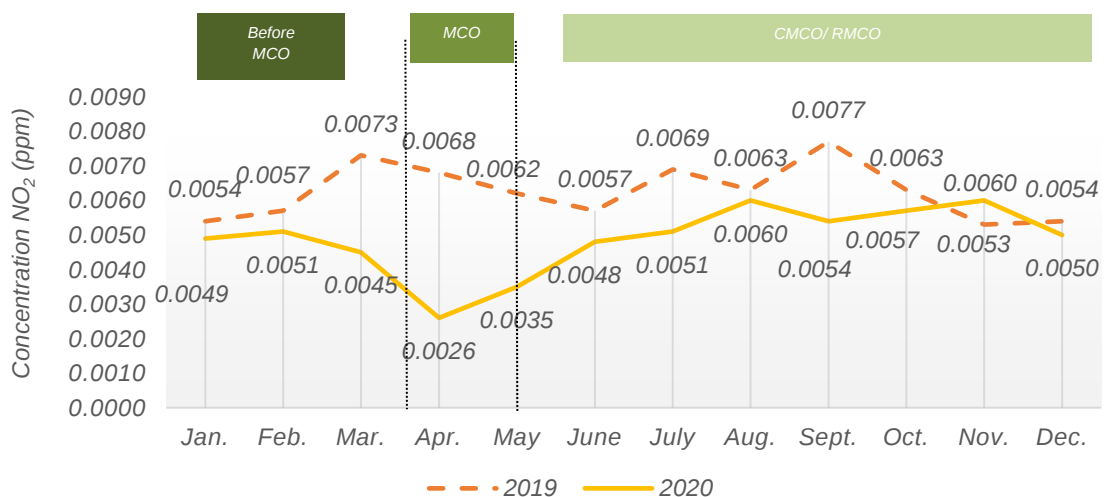
Chart 1.25: Monthly average concentration of NO 2 in the air, Tanjung Malim station, Perak, 2019 and 2020
