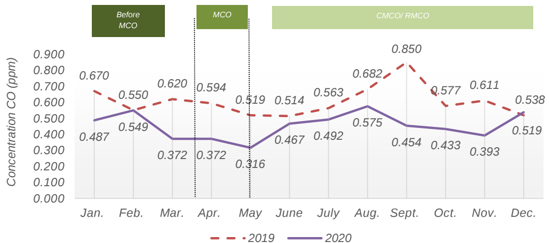
Chart 1.15: Monthly average concentration of CO in the air, Pegoh, Ipoh station, Perak, 2019 and 2020
