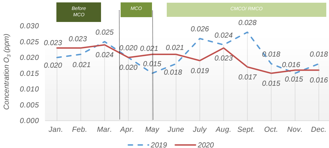
Chart 1.14: Monthly average concentration of O 3 in the air, Tasek, Ipoh station, Perak, 2019 and 2020
