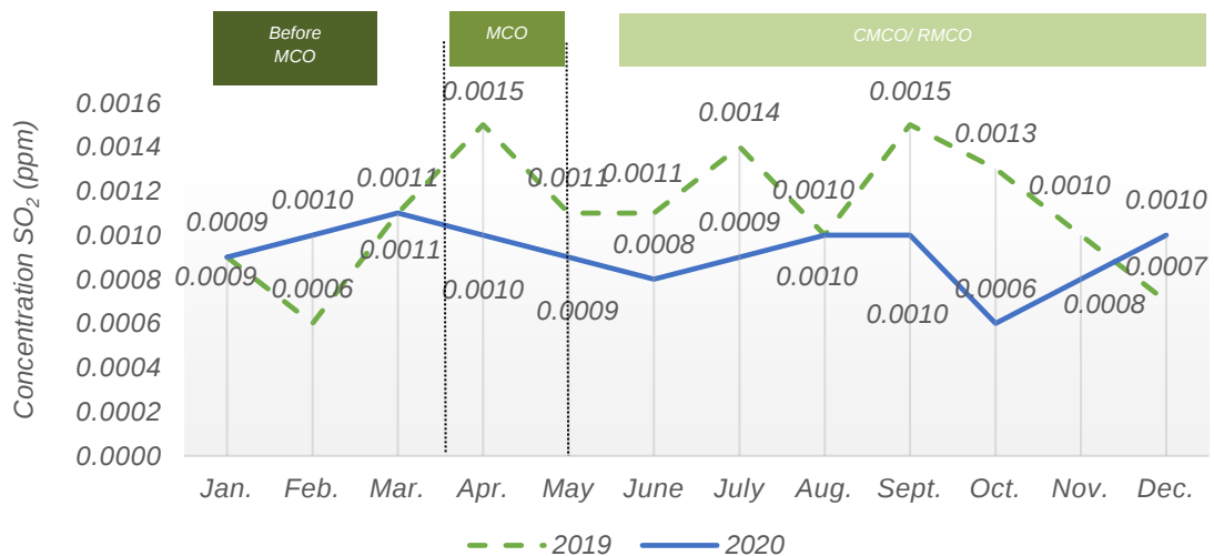
Chart 1.20: Monthly average concentration of SO 2 in the air, Taiping station, Perak, 2019 and 2020
