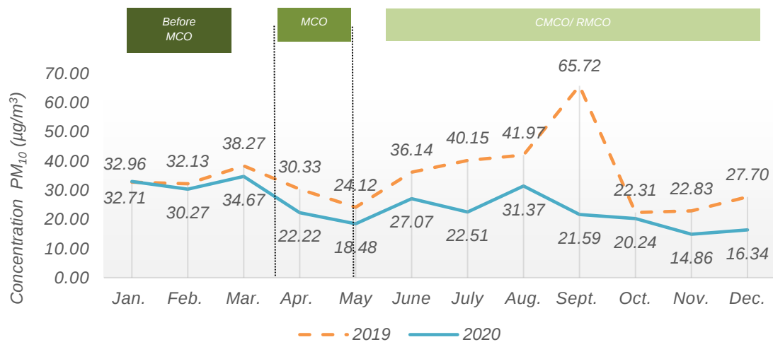
Chart 1.3: Monthly average concentration of PM 10 in the air, Taiping station, Perak, 2019 and 2020
