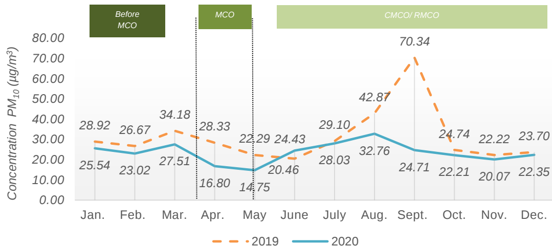
Chart 1.5: Monthly average concentration of PM_{10} in the air, Tasek, Ipoh station, Perak, 2019 and 2020
