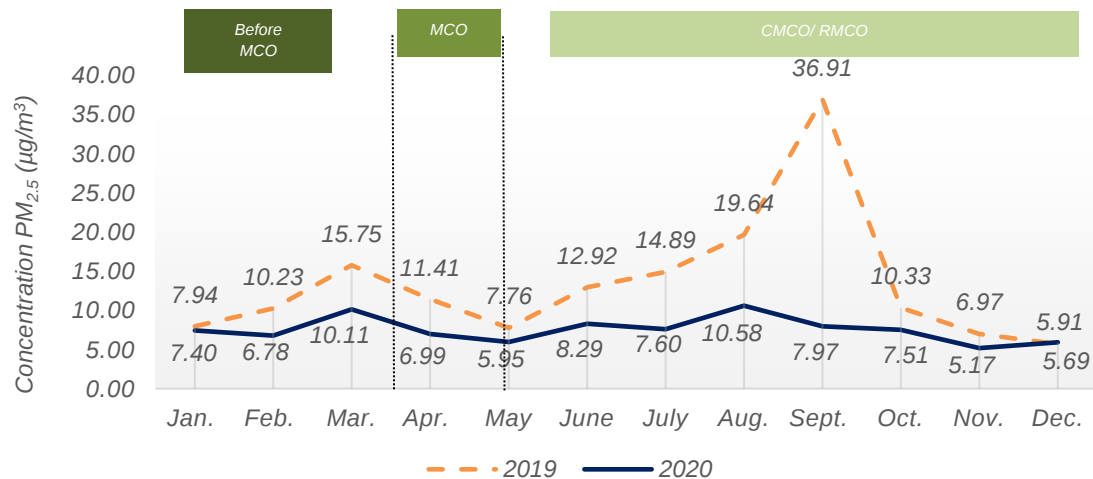
Chart 1.9: Monthly average concentration of PM 2.5 in the air, Tanjung Malim station, Perak, 2019 and 2020
