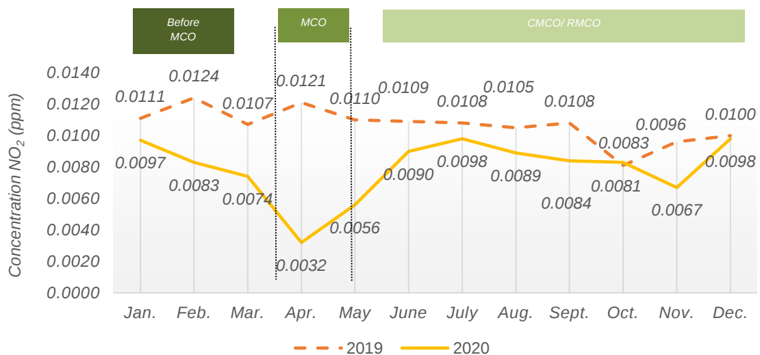
Chart 1.26: Monthly average concentration of NO 2 in the air, Tasek, Ipoh station, Perak, 2019 and 2020
