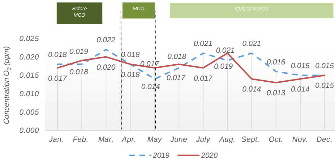
Chart 1.12: Monthly average concentration of O 3 in the air, Taiping station, Perak, 2019 and 2020
