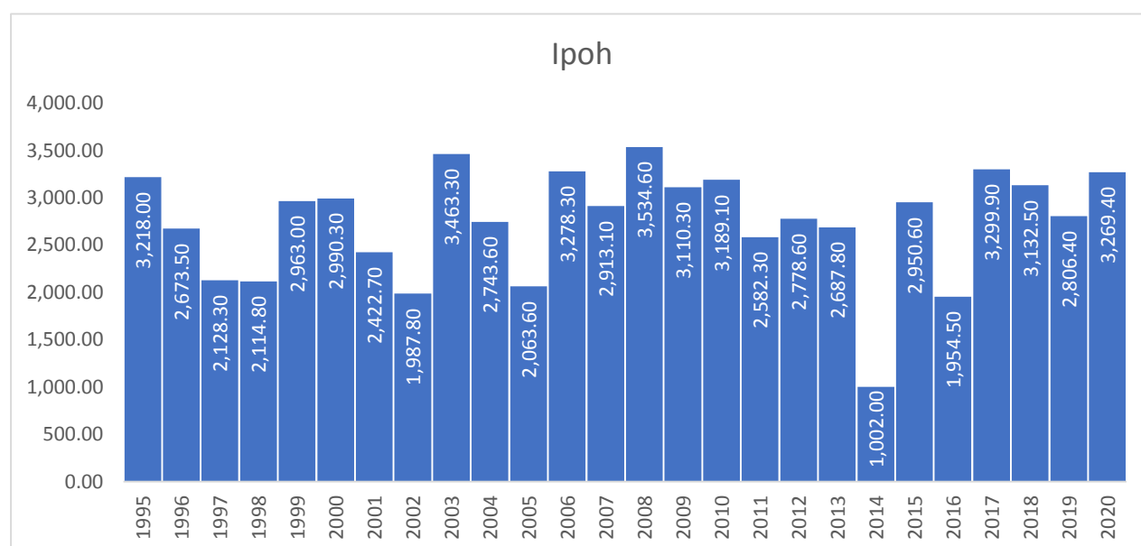
Chart 1.1: Rainfall distribution at Ipoh meteorological station, Perak, 1995-2020
