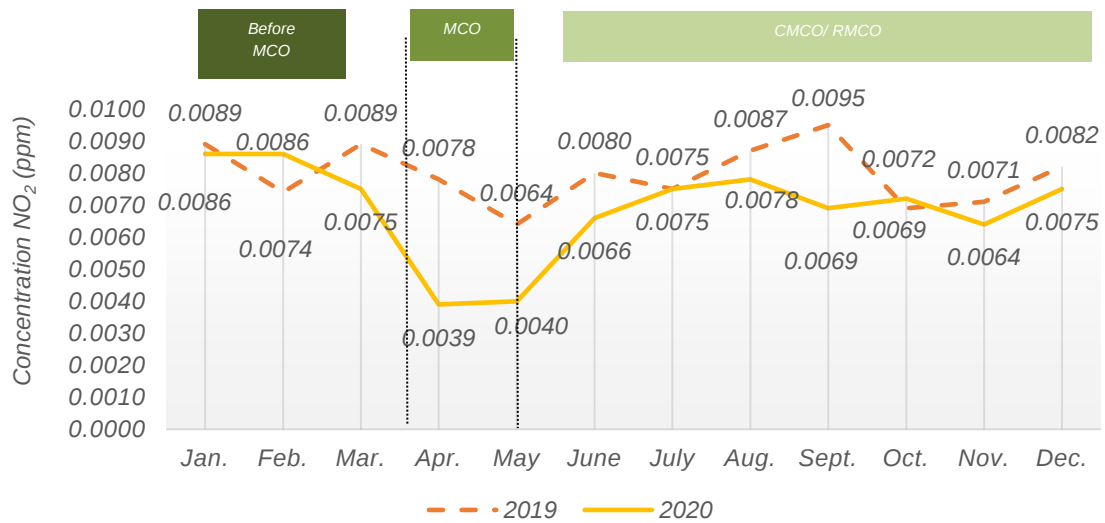
Chart 1.24: Monthly average concentration of NO 2 in the air, Taiping station, Perak, 2019 and 2020
