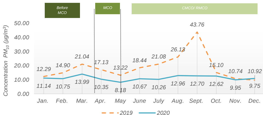
Chart 1.4: Monthly average concentration of PM 10 in the air, Tanjung Malim station, Perak, 2019 and 2020
