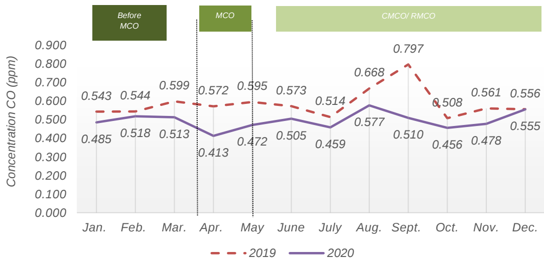
Chart 1.17: Monthly average concentration of CO in the air, Tanjung Malim station, Perak, 2019 and 2020
