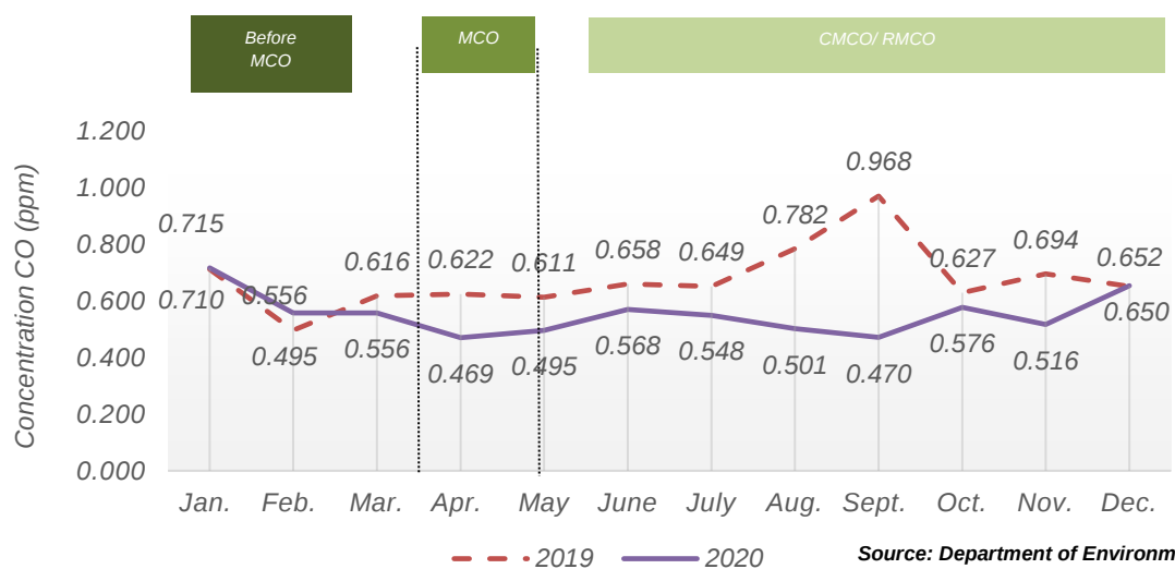
Chart 1.18: Monthly average concentration of CO in the air, Tasek, Ipoh station, Perak, 2019 and 2020
