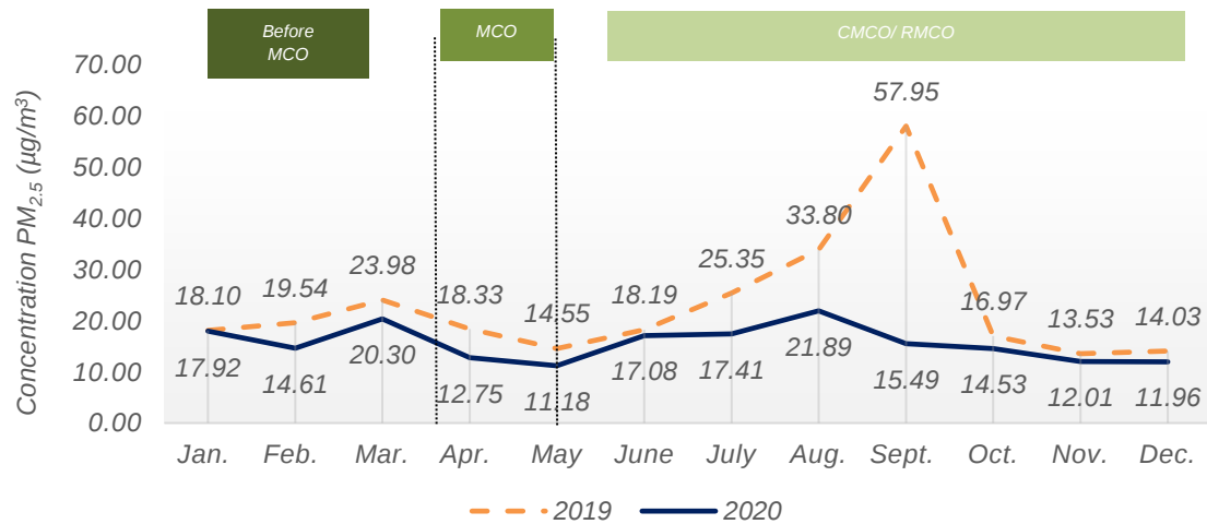
Chart 1.10: Monthly average concentration of PM 2.5 in the air, Tasek, Ipoh station, Perak, 2019 and 2020
