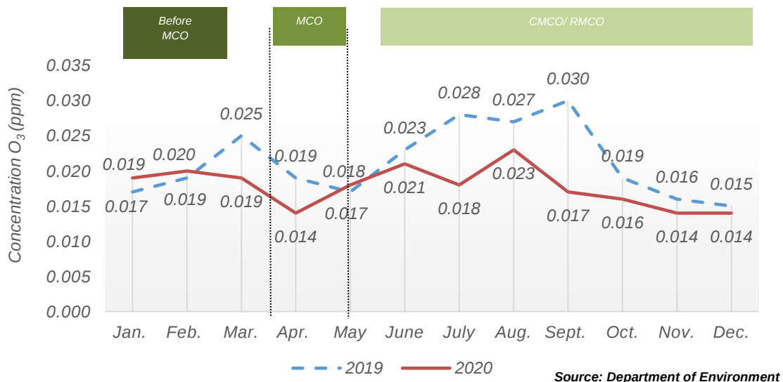
Chart 1.13: Monthly average concentration of O 3 in the air, Tanjung Malim station, Perak, 2019 and 2020
