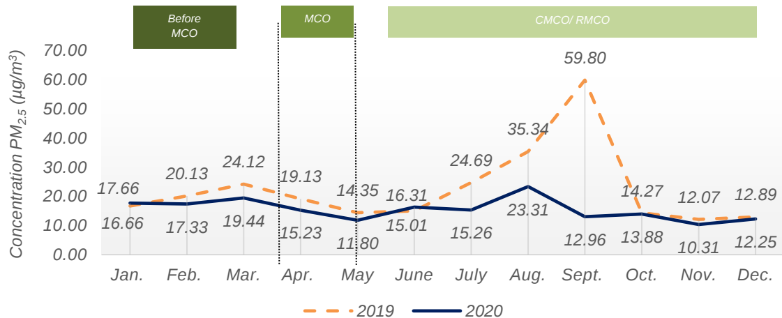
Chart 1.7: Monthly average concentration of PM 2.5 in the air, Seri Manjung station, Perak, 2019 and 2020
